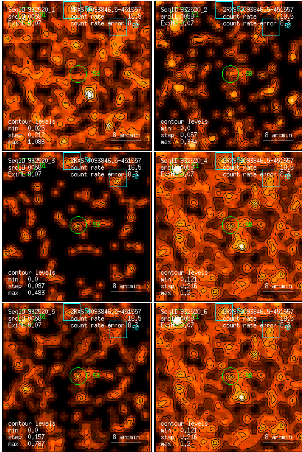
Figure 58: RASS 932520: detection 0058: band rate images, Gaussian filter: (1) PSPC channels 11 – 41, (2) 52 – 90, (3) 91 – 201, (4) 11 – 235, (5) 52 – 201, (6) 11 – 201. Broad band rates in counts/ks. Band rate contour levels in counts/ks/arcmin 2 .
