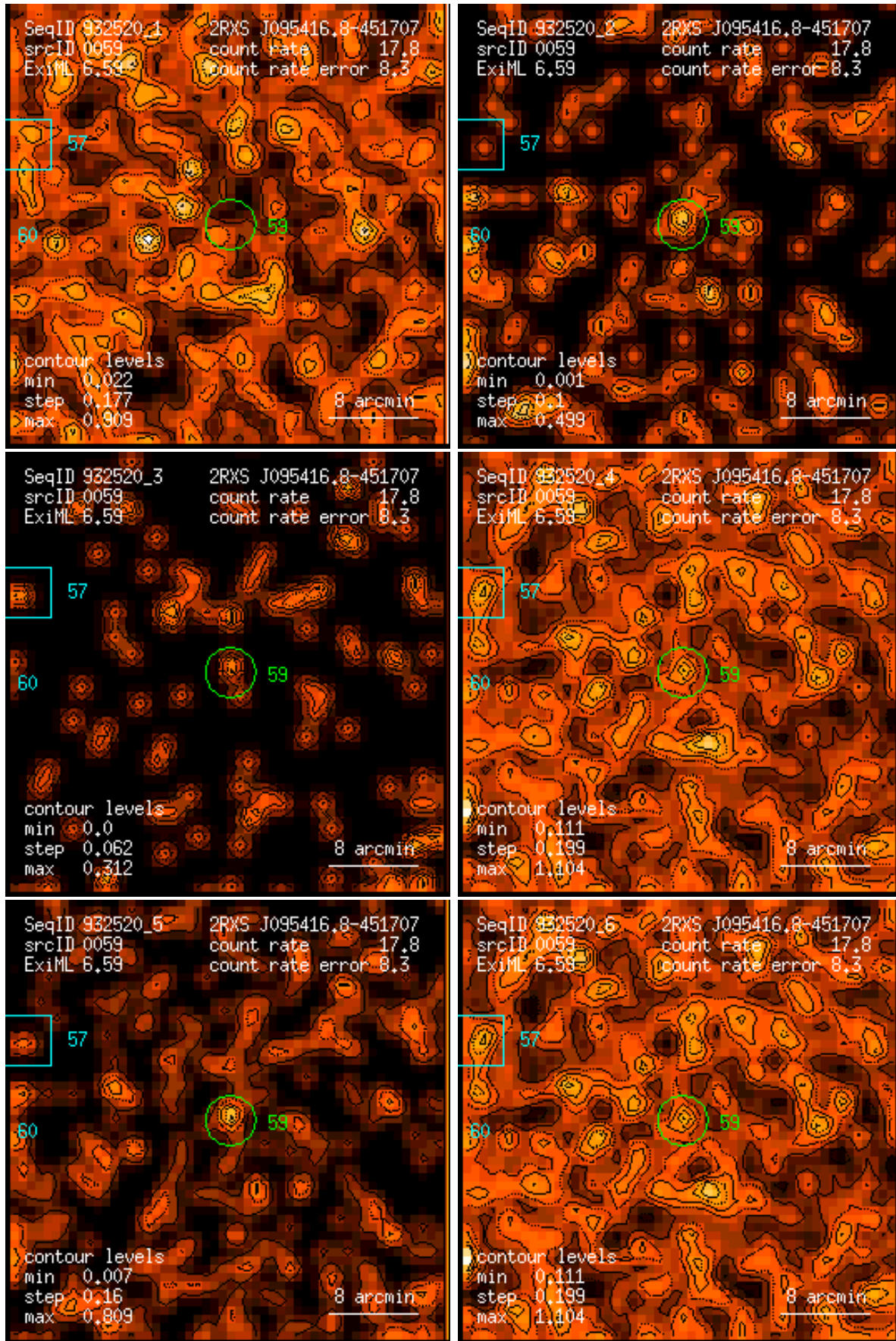
Figure 59: RASS 932520: detection 0059: band rate images, Gaussian filter: (1) PSPC channels 11 – 41, (2) 52 – 90, (3) 91 – 201, (4) 11 – 235, (5) 52 – 201, (6) 11 – 201. Broad band rates in counts/ks. Band rate contour levels in counts/ks/arcmin 2 .
