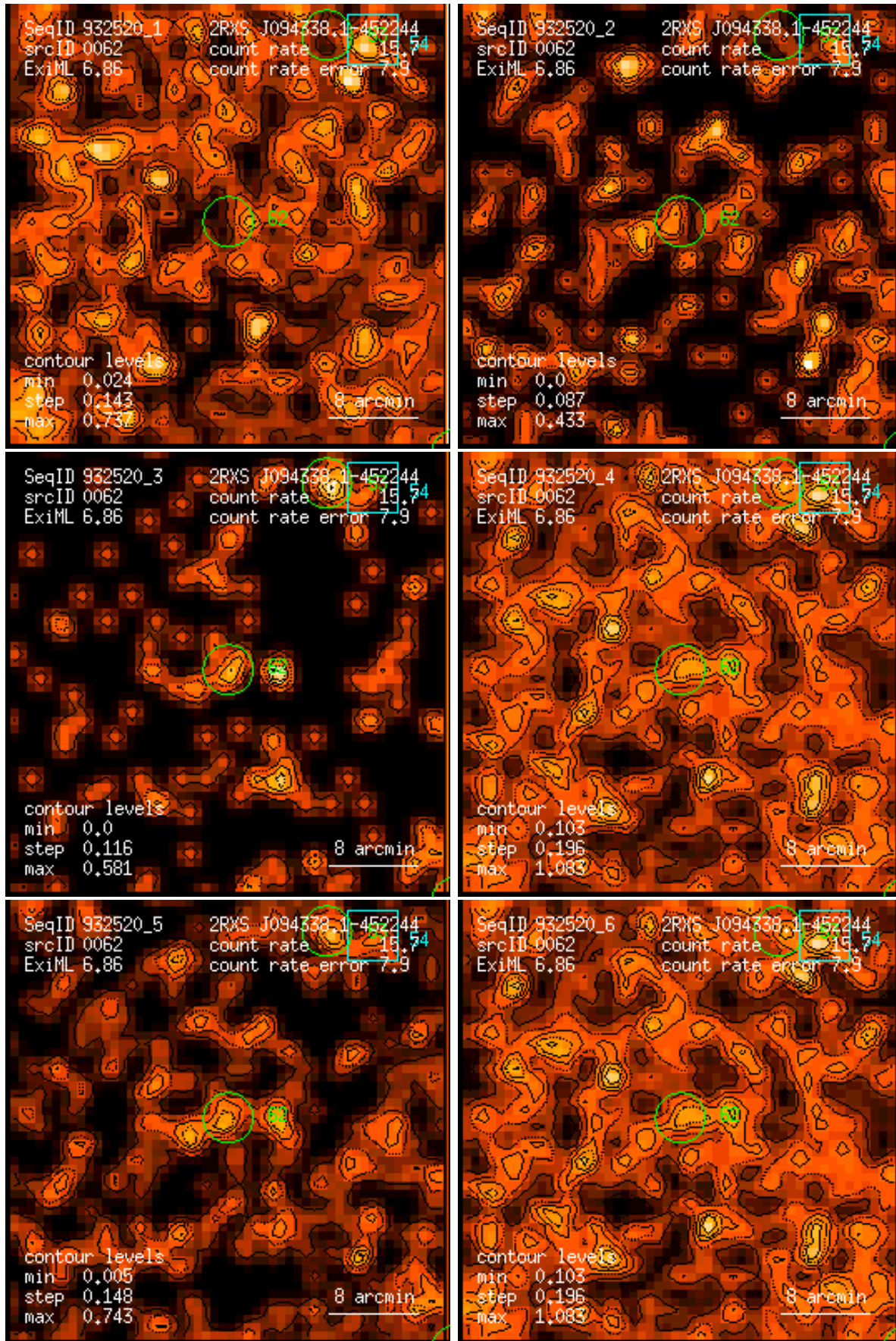
Figure 62: RASS 932520: detection 0062: band rate images, Gaussian filter: (1) PSPC channels 11 – 41, (2) 52 – 90, (3) 91 – 201, (4) 11 – 235, (5) 52 – 201, (6) 11 – 201. Broad band rates in counts/ks. Band rate contour levels in counts/ks/arcmin 2 .
