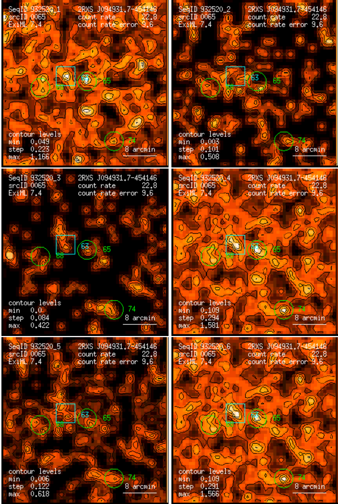
Figure 65: RASS 932520: detection 0065: band rate images, Gaussian filter: (1) PSPC channels 11 – 41, (2) 52 – 90, (3) 91 – 201, (4) 11 – 235, (5) 52 – 201, (6) 11 – 201. Broad band rates in counts/ks. Band rate contour levels in counts/ks/arcmin 2 .
