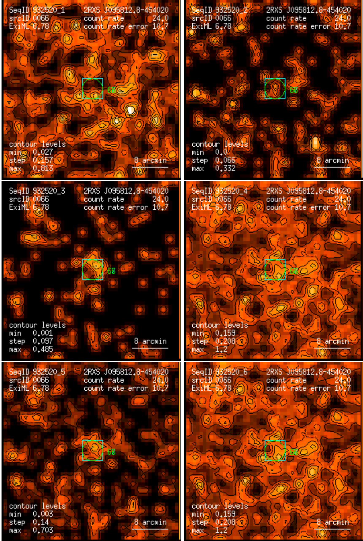
Figure 66: RASS 932520: detection 0066: band rate images, Gaussian filter: (1) PSPC channels 11 – 41, (2) 52 – 90, (3) 91 – 201, (4) 11 – 235, (5) 52 – 201, (6) 11 – 201. Broad band rates in counts/ks. Band rate contour levels in counts/ks/arcmin 2 .
