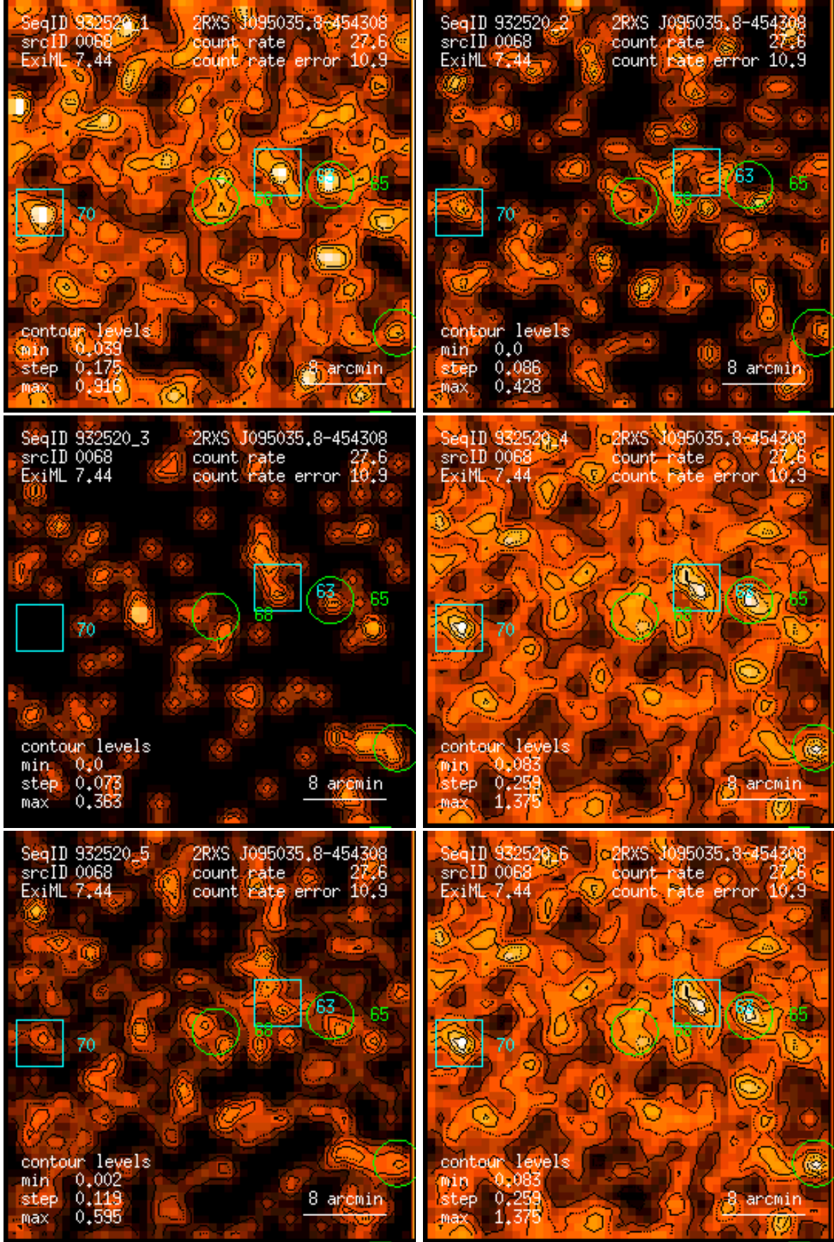
Figure 68: RASS 932520: detection 0068: band rate images, Gaussian filter: (1) PSPC channels 11 – 41, (2) 52 – 90, (3) 91 – 201, (4) 11 – 235, (5) 52 – 201, (6) 11 – 201. Broad band rates in counts/ks. Band rate contour levels in counts/ks/arcmin 2 .
