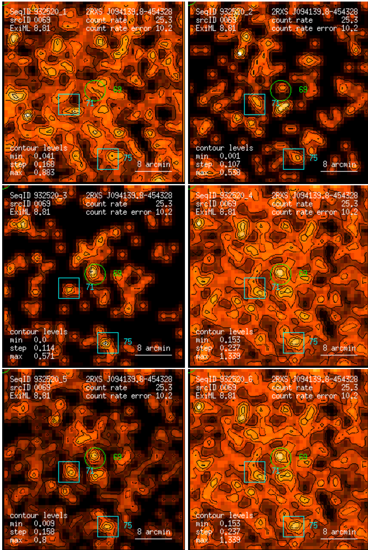
Figure 69: RASS 932520: detection 0069: band rate images, Gaussian filter: (1) PSPC channels 11 – 41, (2) 52 – 90, (3) 91 – 201, (4) 11 – 235, (5) 52 – 201, (6) 11 – 201. Broad band rates in counts/ks. Band rate contour levels in counts/ks/arcmin 2 .
