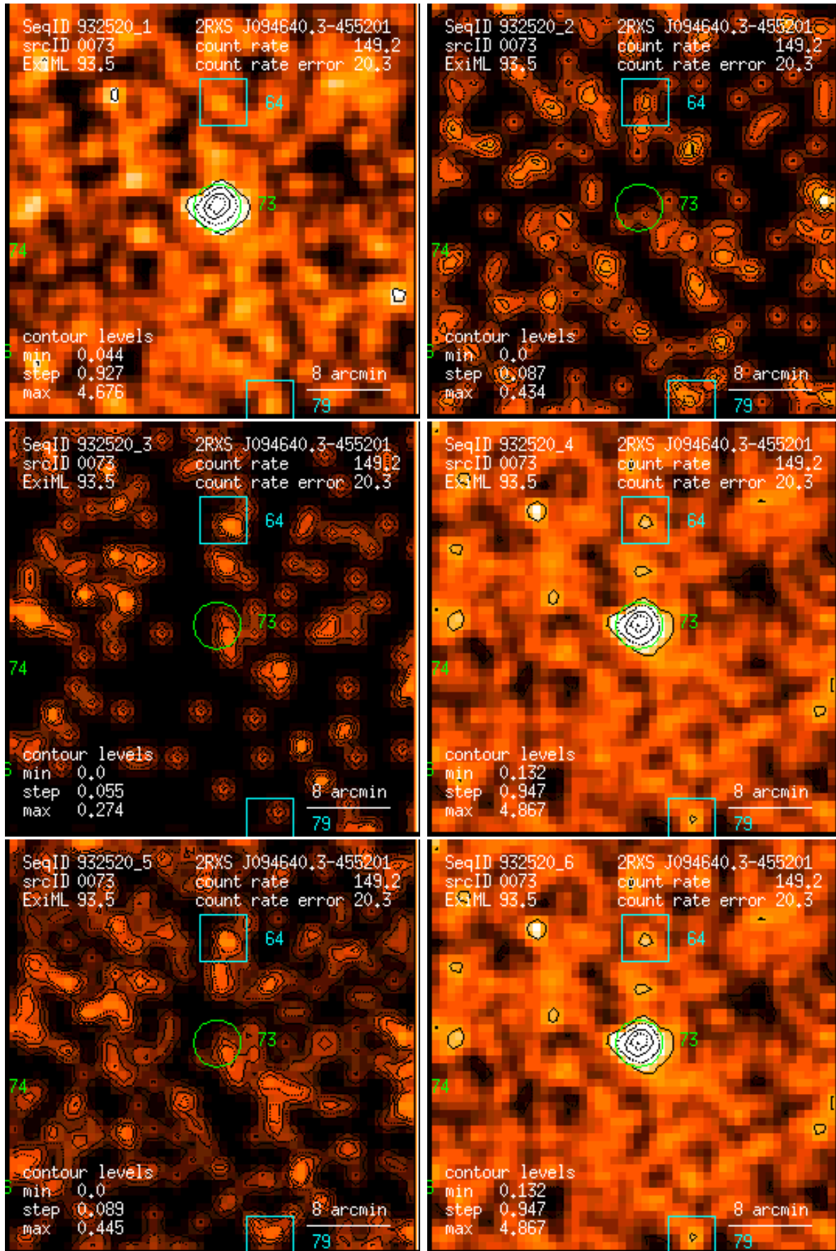
Figure 73: RASS 932520: detection 0073: band rate images, Gaussian filter: (1) PSPC channels 11 – 41, (2) 52 – 90, (3) 91 – 201, (4) 11 – 235, (5) 52 – 201, (6) 11 – 201. Broad band rates in counts/ks. Band rate contour levels in counts/ks/arcmin 2 .
