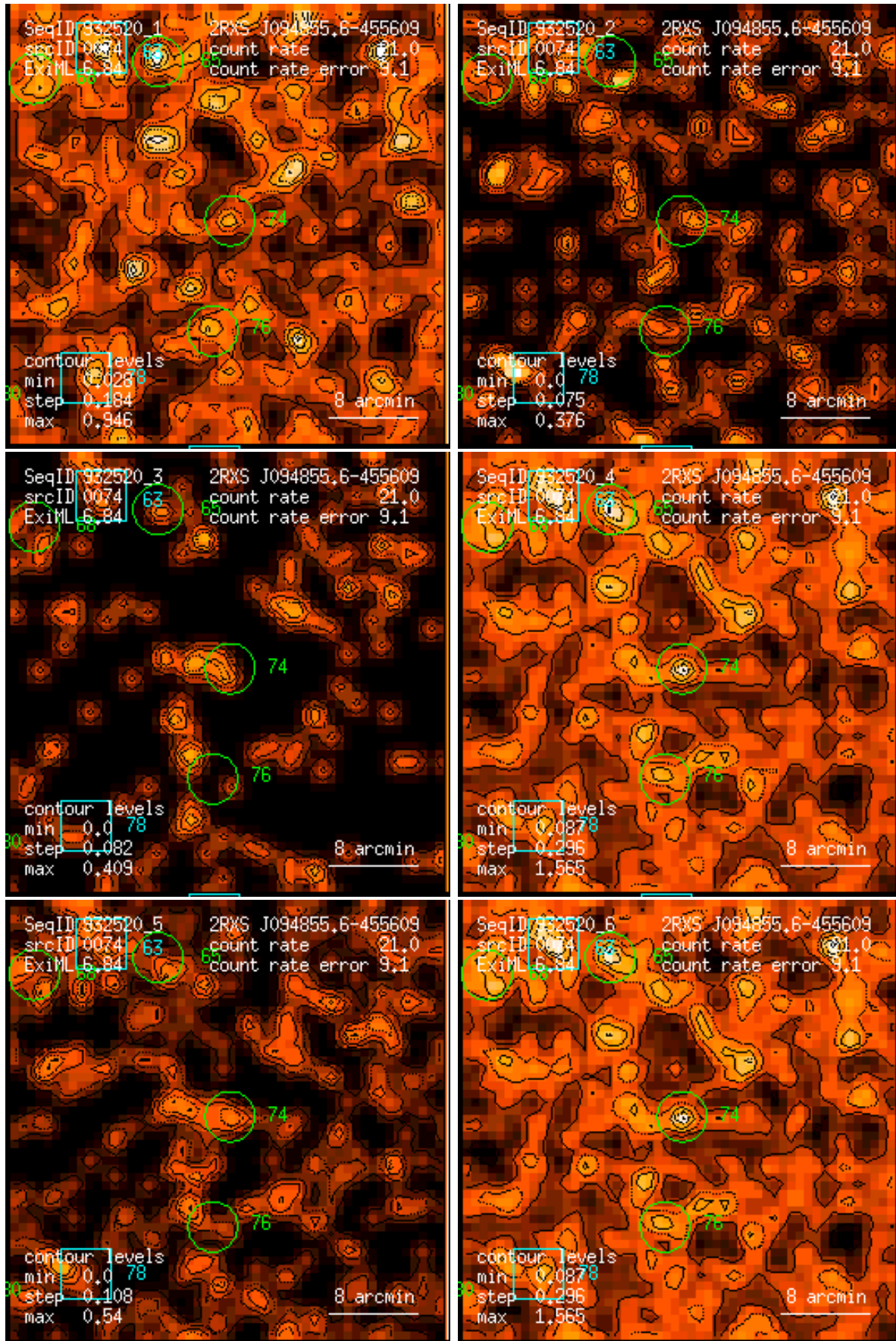
Figure 74: RASS 932520: detection 0074: band rate images, Gaussian filter: (1) PSPC channels 11 – 41, (2) 52 – 90, (3) 91 – 201, (4) 11 – 235, (5) 52 – 201, (6) 11 – 201. Broad band rates in counts/ks. Band rate contour levels in counts/ks/arcmin 2 .
