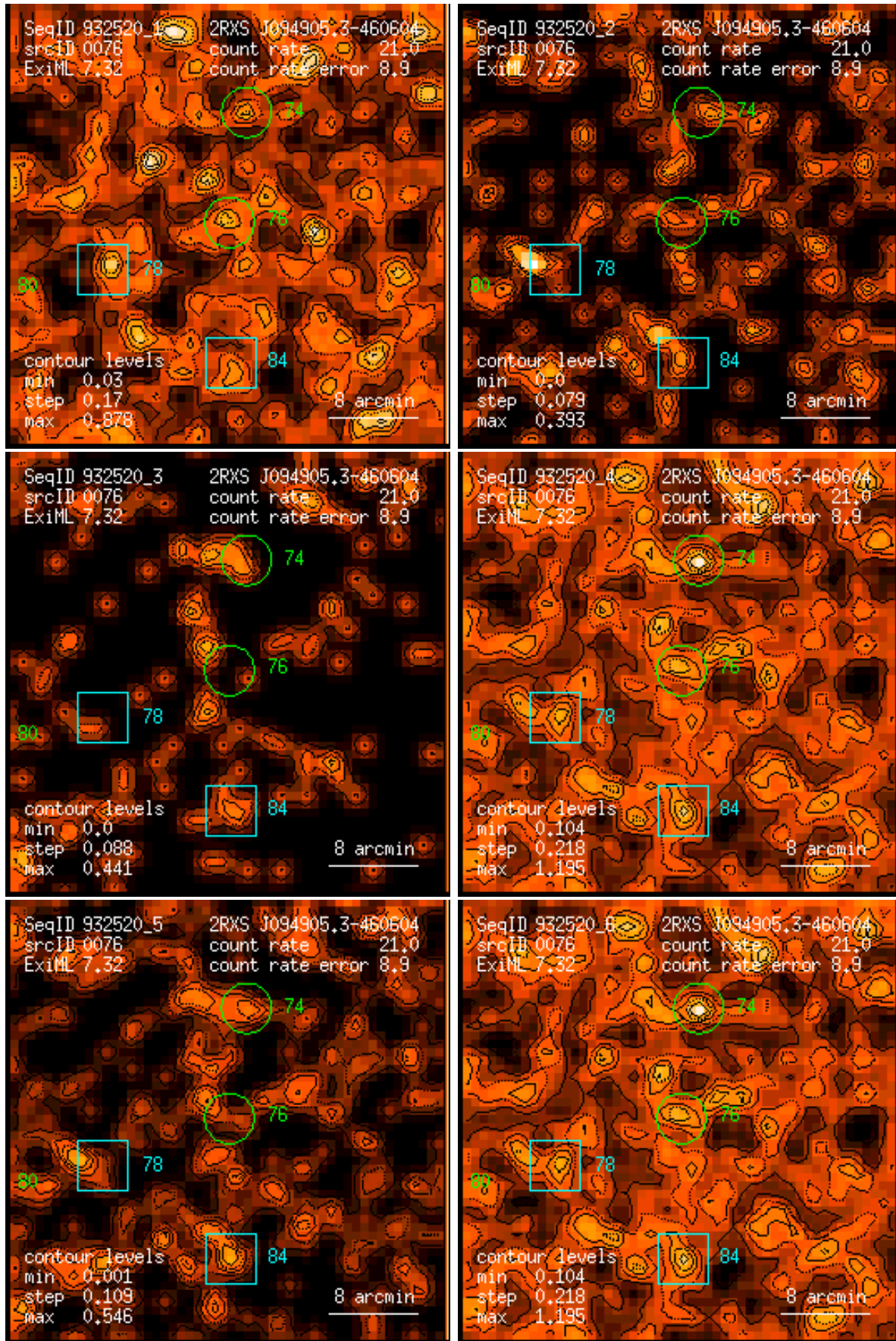
Figure 76: RASS 932520: detection 0076: band rate images, Gaussian filter: (1) PSPC channels 11 – 41, (2) 52 – 90, (3) 91 – 201, (4) 11 – 235, (5) 52 – 201, (6) 11 – 201. Broad band rates in counts/ks. Band rate contour levels in counts/ks/arcmin 2 .
