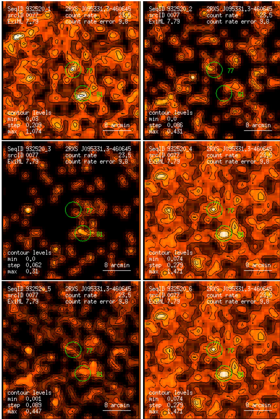
Figure 77: RASS 932520: detection 0077: band rate images, Gaussian filter: (1) PSPC channels 11 – 41, (2) 52 – 90, (3) 91 – 201, (4) 11 – 235, (5) 52 – 201, (6) 11 – 201. Broad band rates in counts/ks. Band rate contour levels in counts/ks/arcmin 2 .
