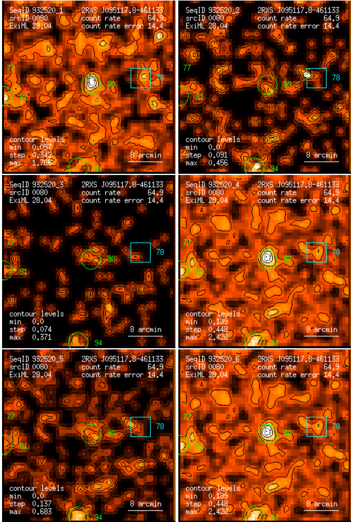
Figure 80: RASS 932520: detection 0080: band rate images, Gaussian filter: (1) PSPC channels 11 – 41, (2) 52 – 90, (3) 91 – 201, (4) 11 – 235, (5) 52 – 201, (6) 11 – 201. Broad band rates in counts/ks. Band rate contour levels in counts/ks/arcmin 2 .
