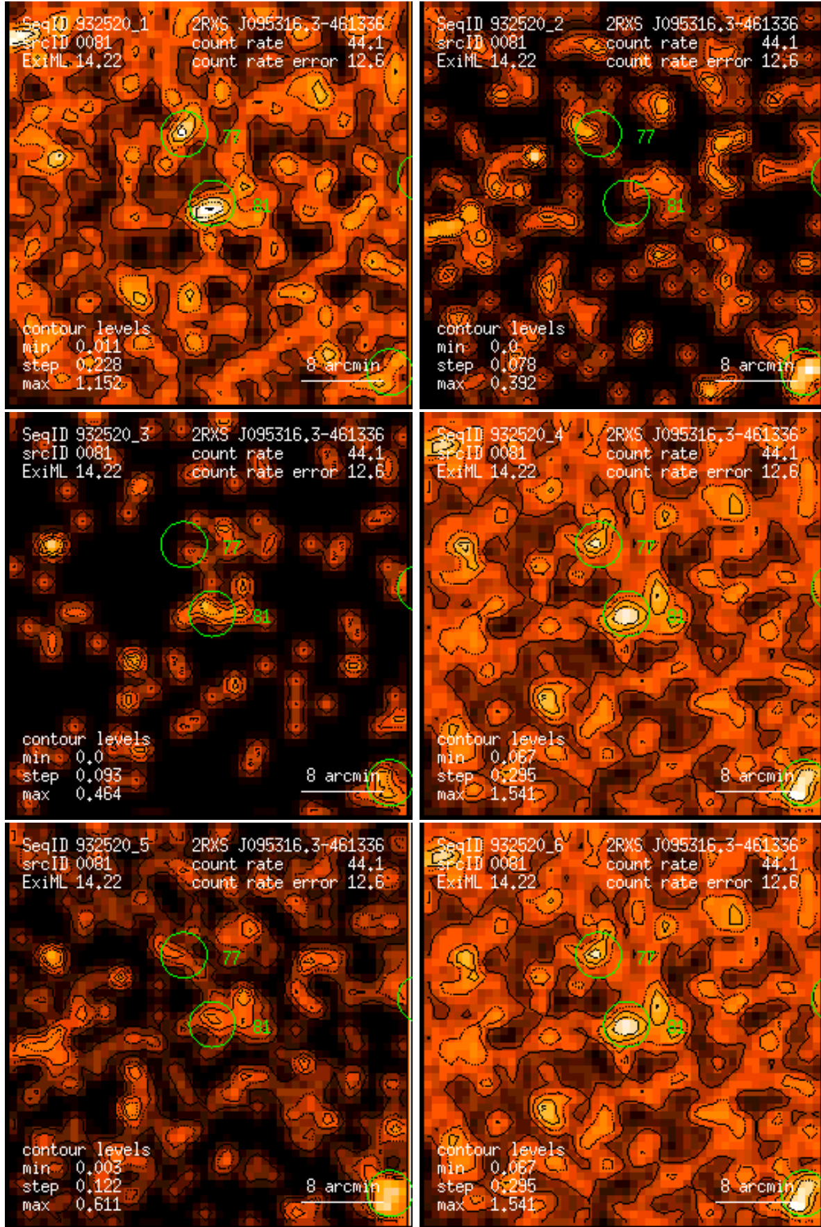
Figure 81: RASS 932520: detection 0081: band rate images, Gaussian filter: (1) PSPC channels 11 – 41, (2) 52 – 90, (3) 91 – 201, (4) 11 – 235, (5) 52 – 201, (6) 11 – 201. Broad band rates in counts/ks. Band rate contour levels in counts/ks/arcmin 2 .
