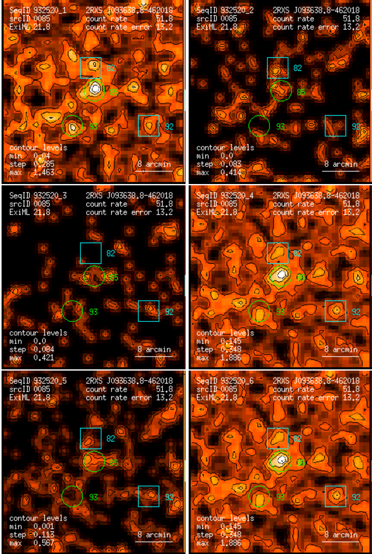
Figure 85: RASS 932520: detection 0085: band rate images, Gaussian filter: (1) PSPC channels 11 – 41, (2) 52 – 90, (3) 91 – 201, (4) 11 – 235, (5) 52 – 201, (6) 11 – 201. Broad band rates in counts/ks. Band rate contour levels in counts/ks/arcmin 2 .
