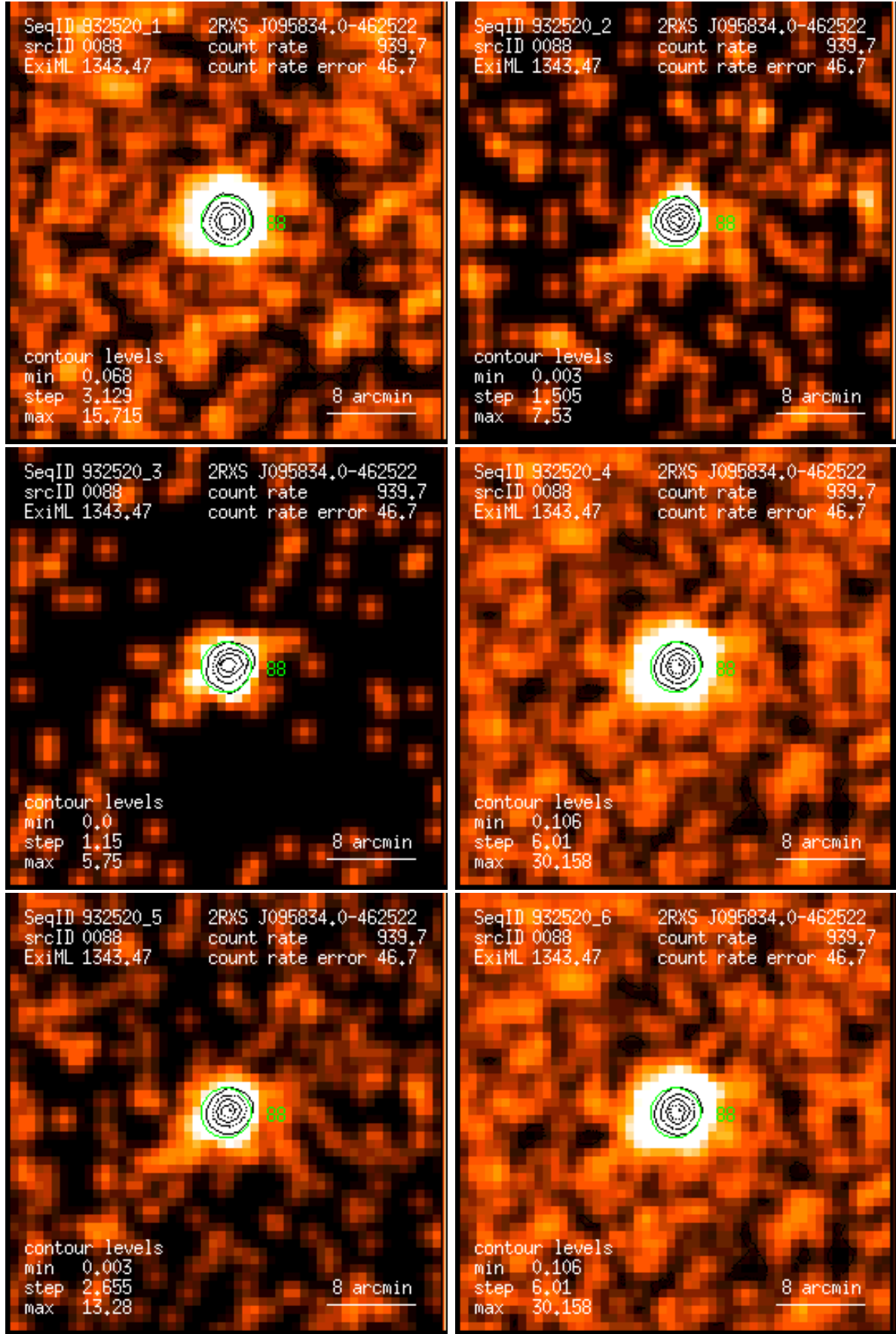
Figure 88: RASS 932520: detection 0088: band rate images, Gaussian filter: (1) PSPC channels 11 – 41, (2) 52 – 90, (3) 91 – 201, (4) 11 – 235, (5) 52 – 201, (6) 11 – 201. Broad band rates in counts/ks. Band rate contour levels in counts/ks/arcmin 2 .
