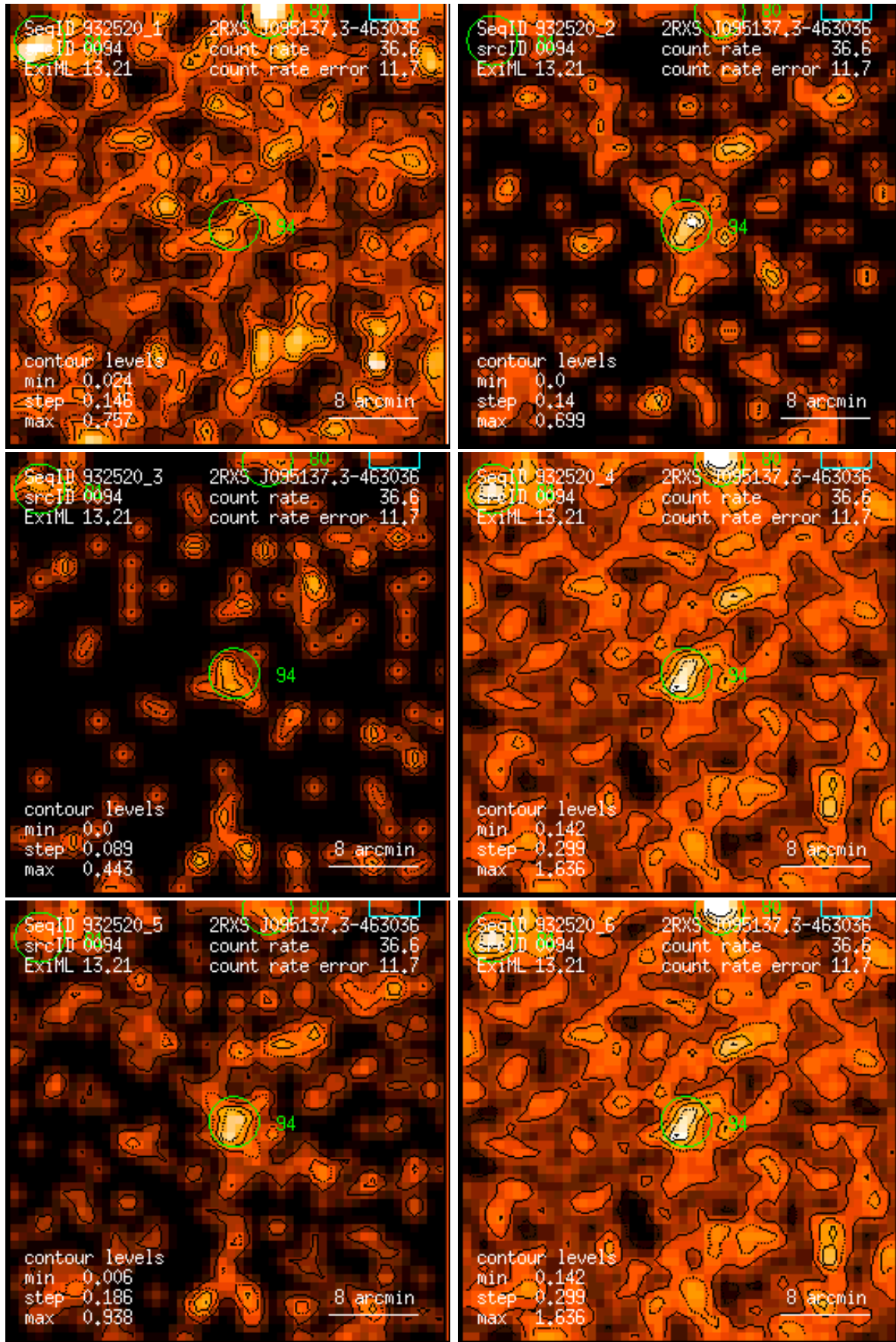
Figure 94: RASS 932520: detection 0094: band rate images, Gaussian filter: (1) PSPC channels 11 – 41, (2) 52 – 90, (3) 91 – 201, (4) 11 – 235, (5) 52 – 201, (6) 11 – 201. Broad band rates in counts/ks. Band rate contour levels in counts/ks/arcmin 2 .
