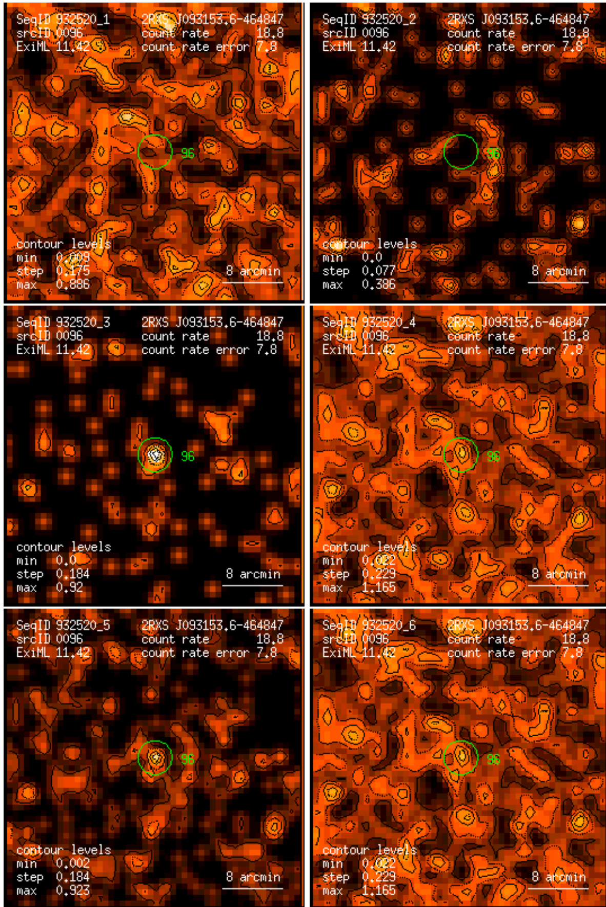
Figure 96: RASS 932520: detection 0096: band rate images, Gaussian filter: (1) PSPC channels 11 – 41, (2) 52 – 90, (3) 91 – 201, (4) 11 – 235, (5) 52 – 201, (6) 11 – 201. Broad band rates in counts/ks. Band rate contour levels in counts/ks/arcmin 2 .
