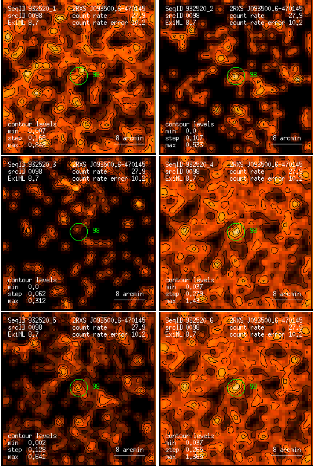
Figure 98: RASS 932520: detection 0098: band rate images, Gaussian filter: (1) PSPC channels 11 – 41, (2) 52 – 90, (3) 91 – 201, (4) 11 – 235, (5) 52 – 201, (6) 11 – 201. Broad band rates in counts/ks. Band rate contour levels in counts/ks/arcmin 2 .
