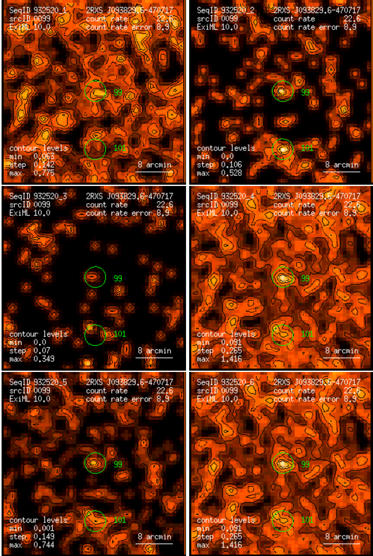
Figure 99: RASS 932520: detection 0099: band rate images, Gaussian filter: (1) PSPC channels 11 – 41, (2) 52 – 90, (3) 91 – 201, (4) 11 – 235, (5) 52 – 201, (6) 11 – 201. Broad band rates in counts/ks. Band rate contour levels in counts/ks/arcmin 2 .
