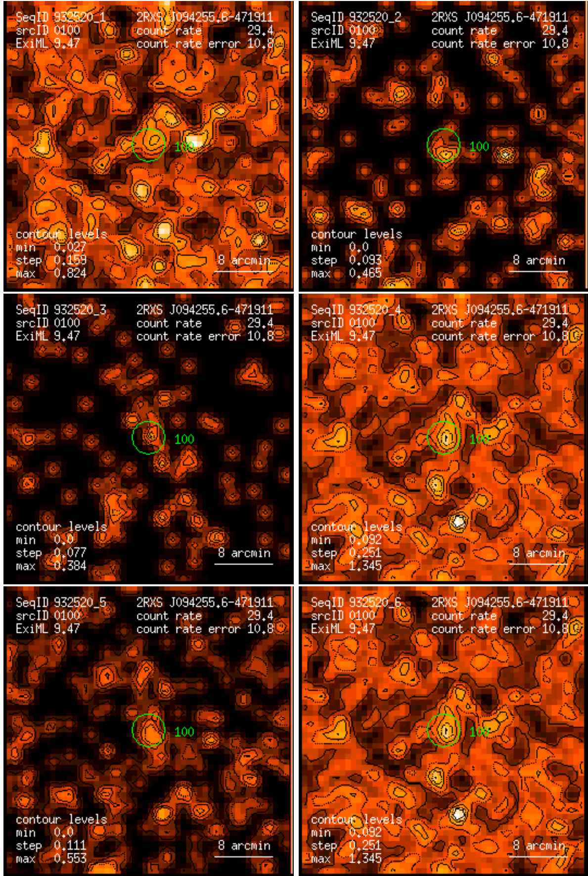
Figure 100: RASS 932520: detection 0100: band rate images, Gaussian filter: (1) PSPC channels 11 – 41, (2) 52 – 90, (3) 91 – 201, (4) 11 – 235, (5) 52 – 201, (6) 11 – 201. Broad band rates in counts/ks. Band rate contour levels in counts/ks/arcmin 2 .
