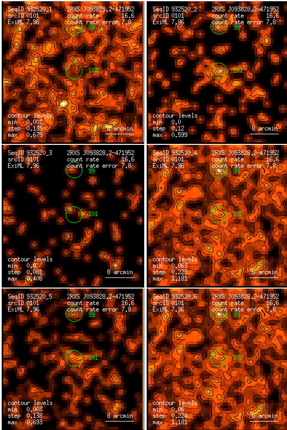
Figure 101: RASS 932520: detection 0101: band rate images, Gaussian filter: (1) PSPC channels 11 – 41, (2) 52 – 90, (3) 91 – 201, (4) 11 – 235, (5) 52 – 201, (6) 11 – 201. Broad band rates in counts/ks. Band rate contour levels in counts/ks/arcmin 2 .
