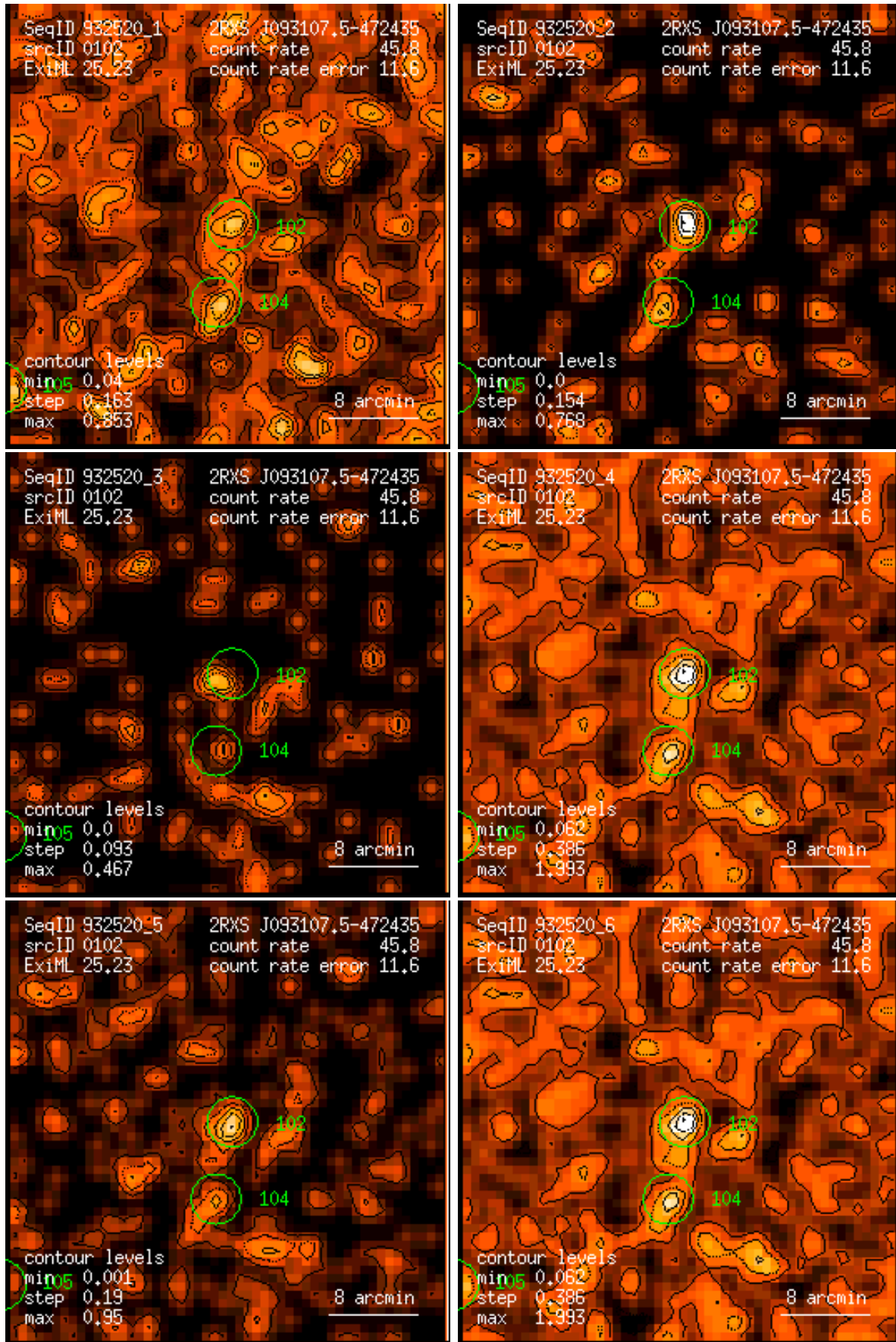
Figure 102: RASS 932520: detection 0102: band rate images, Gaussian filter: (1) PSPC channels 11 – 41, (2) 52 – 90, (3) 91 – 201, (4) 11 – 235, (5) 52 – 201, (6) 11 – 201. Broad band rates in counts/ks. Band rate contour levels in counts/ks/arcmin 2 .
