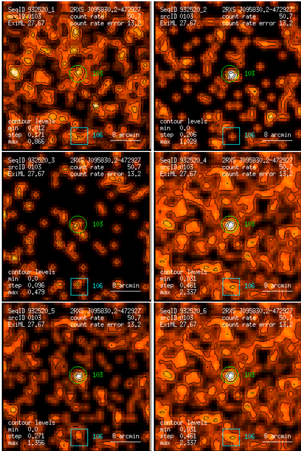
Figure 103: RASS 932520: detection 0103: band rate images, Gaussian filter: (1) PSPC channels 11 – 41, (2) 52 – 90, (3) 91 – 201, (4) 11 – 235, (5) 52 – 201, (6) 11 – 201. Broad band rates in counts/ks. Band rate contour levels in counts/ks/arcmin 2 .
