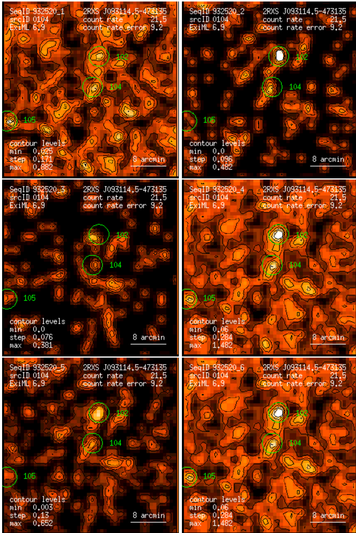
Figure 104: RASS 932520: detection 0104: band rate images, Gaussian filter: (1) PSPC channels 11 – 41, (2) 52 – 90, (3) 91 – 201, (4) 11 – 235, (5) 52 – 201, (6) 11 – 201. Broad band rates in counts/ks. Band rate contour levels in counts/ks/arcmin 2 .
