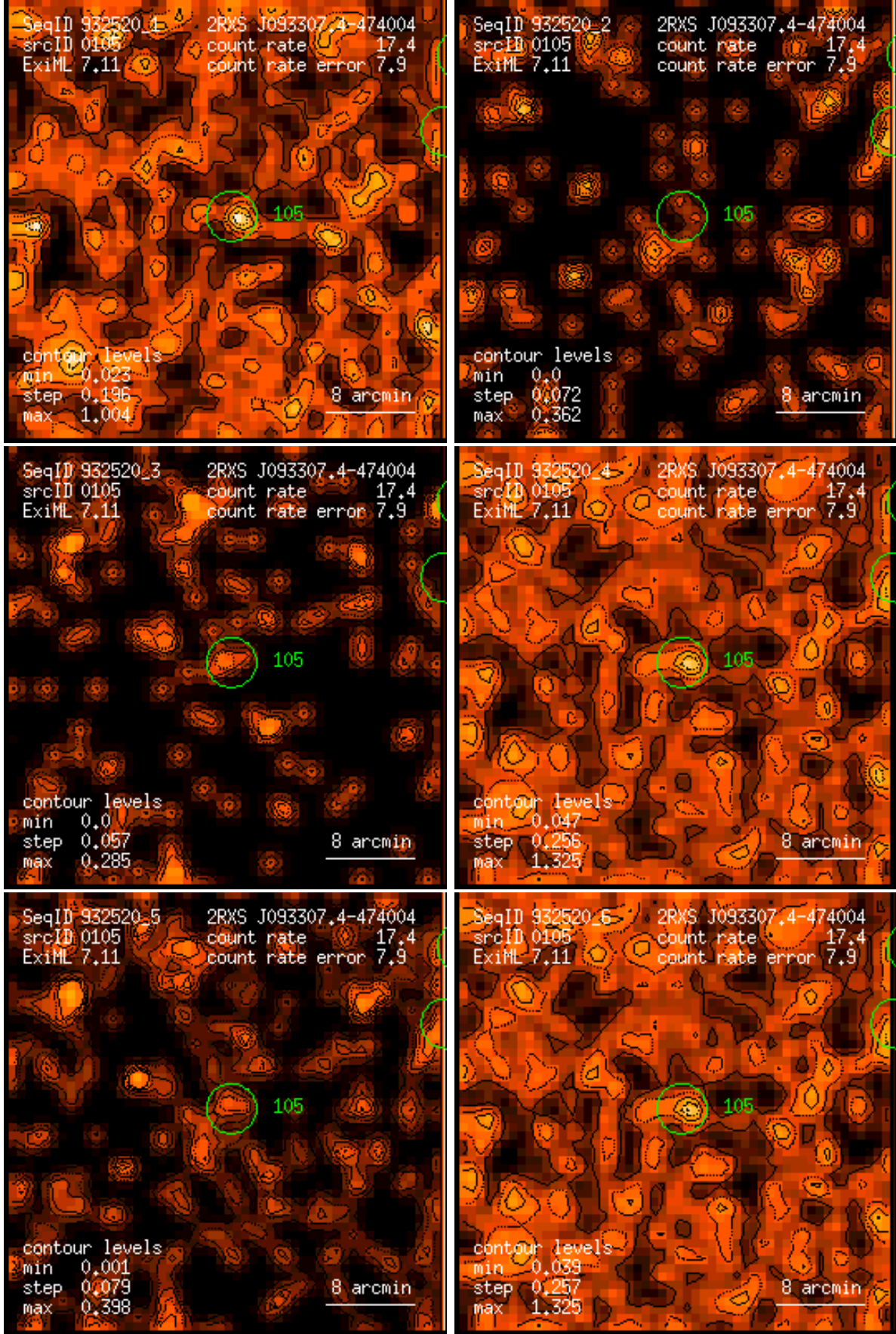
Figure 105: RASS 932520: detection 0105: band rate images, Gaussian filter: (1) PSPC channels 11 – 41, (2) 52 – 90, (3) 91 – 201, (4) 11 – 235, (5) 52 – 201, (6) 11 – 201. Broad band rates in counts/ks. Band rate contour levels in counts/ks/arcmin 2 .
