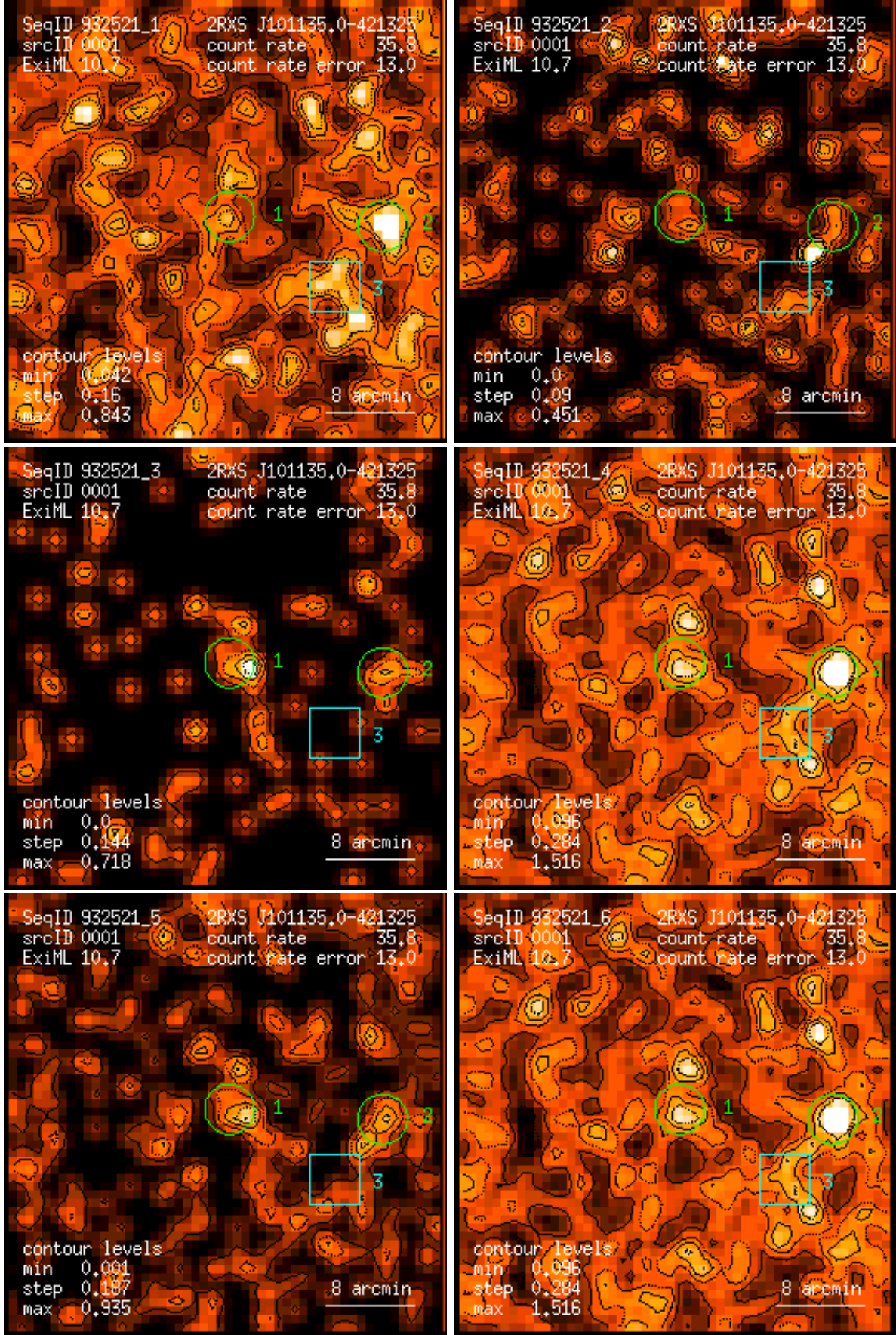
Figure 1: RASS 932521: detection 0001: band rate images, Gaussian filter: (1) PSPC channels 11 – 41, (2) 52 – 90, (3) 91 – 201, (4) 11 – 235, (5) 52 – 201, (6) 11 – 201. Broad band rates in counts/ks. Band rate contour levels in counts/ks/arcmin 2 .
