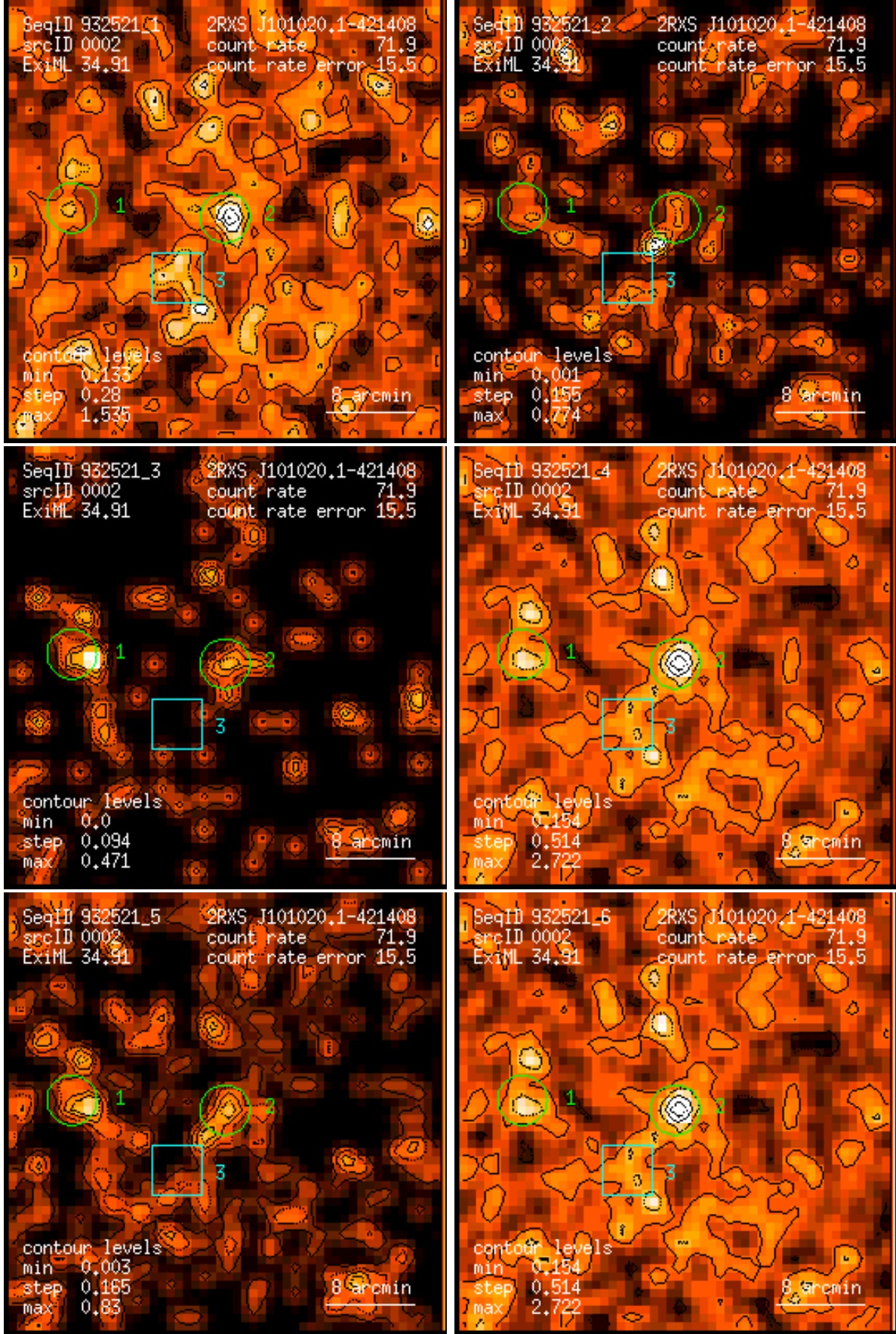
Figure 2: RASS 932521: detection 0002: band rate images, Gaussian filter: (1) PSPC channels 11 – 41, (2) 52 – 90, (3) 91 – 201, (4) 11 – 235, (5) 52 – 201, (6) 11 – 201. Broad band rates in counts/ks. Band rate contour levels in counts/ks/arcmin 2 .
