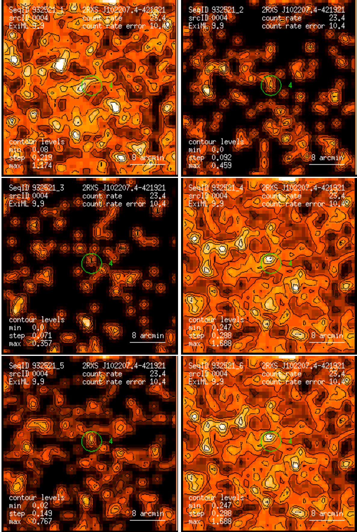
Figure 4: RASS 932521: detection 0004: band rate images, Gaussian filter: (1) PSPC channels 11 – 41, (2) 52 – 90, (3) 91 – 201, (4) 11 – 235, (5) 52 – 201, (6) 11 – 201. Broad band rates in counts/ks. Band rate contour levels in counts/ks/arcmin 2 .
