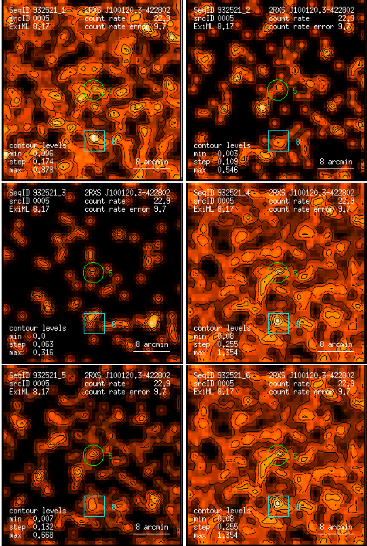
Figure 5: RASS 932521: detection 0005: band rate images, Gaussian filter: (1) PSPC channels 11 – 41, (2) 52 – 90, (3) 91 – 201, (4) 11 – 235, (5) 52 – 201, (6) 11 – 201. Broad band rates in counts/ks. Band rate contour levels in counts/ks/arcmin 2 .
