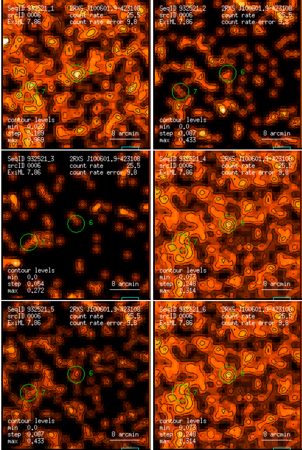
Figure 6: RASS 932521: detection 0006: band rate images, Gaussian filter: (1) PSPC channels 11 – 41, (2) 52 – 90, (3) 91 – 201, (4) 11 – 235, (5) 52 – 201, (6) 11 – 201. Broad band rates in counts/ks. Band rate contour levels in counts/ks/arcmin 2 .
