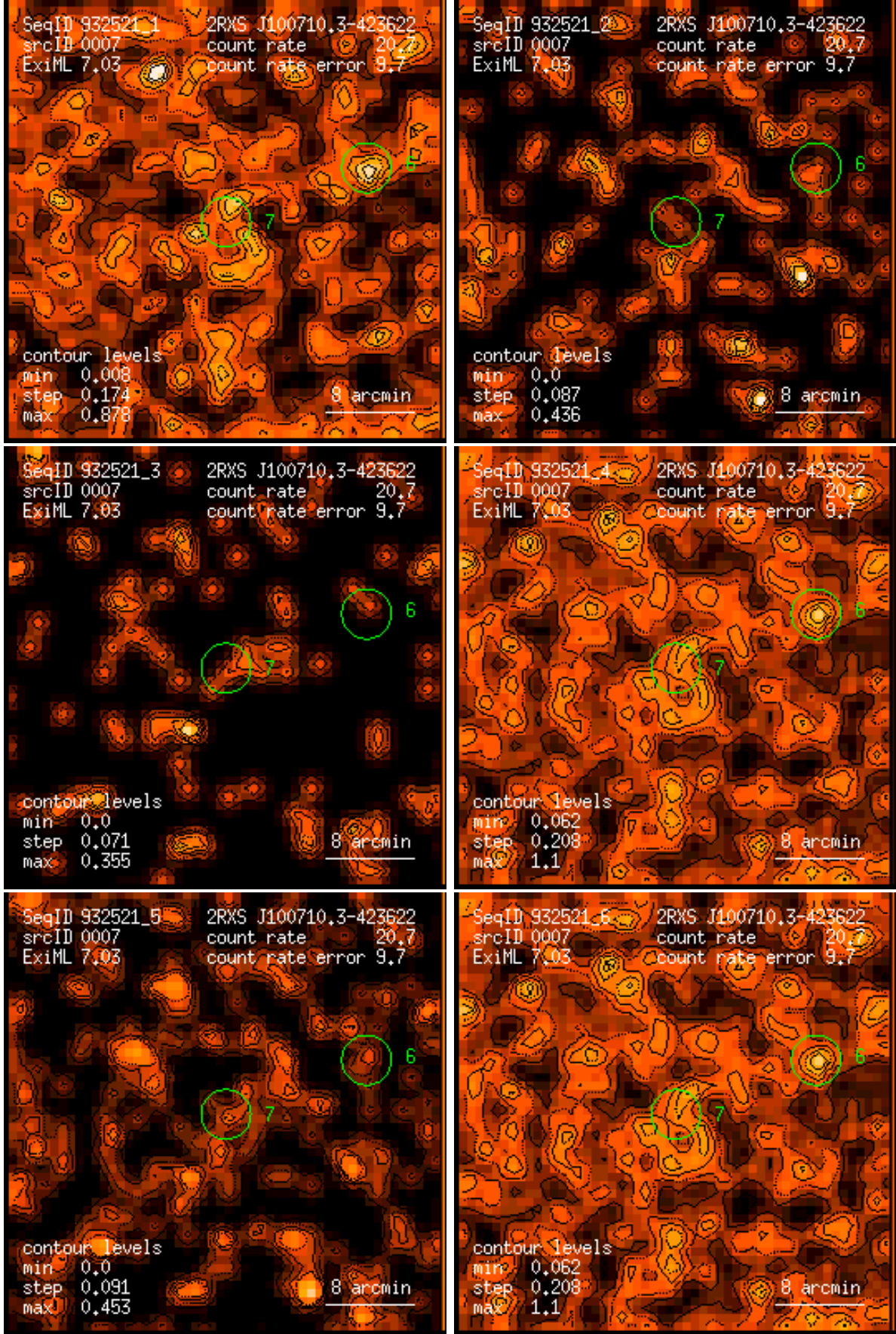
Figure 7: RASS 932521: detection 0007: band rate images, Gaussian filter: (1) PSPC channels 11 – 41, (2) 52 – 90, (3) 91 – 201, (4) 11 – 235, (5) 52 – 201, (6) 11 – 201. Broad band rates in counts/ks. Band rate contour levels in counts/ks/arcmin 2 .
