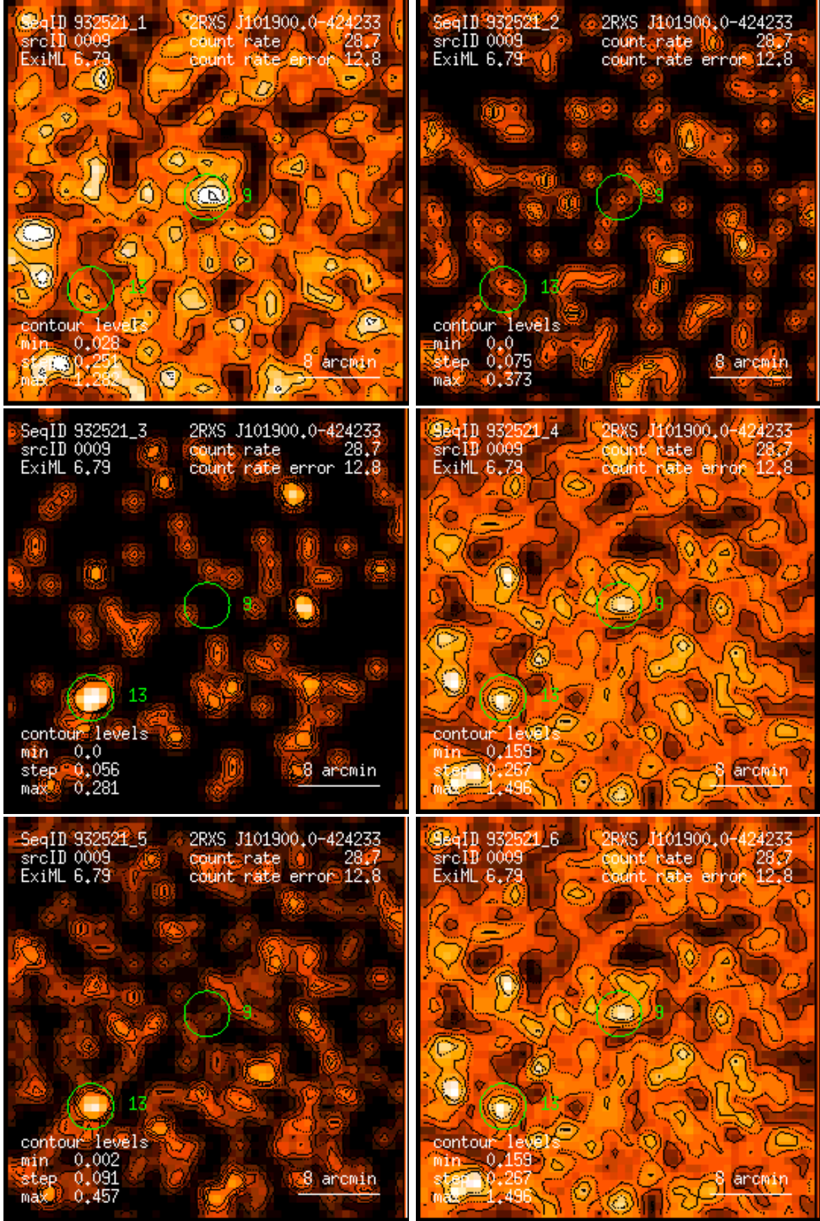
Figure 9: RASS 932521: detection 0009: band rate images, Gaussian filter: (1) PSPC channels 11 – 41, (2) 52 – 90, (3) 91 – 201, (4) 11 – 235, (5) 52 – 201, (6) 11 – 201. Broad band rates in counts/ks. Band rate contour levels in counts/ks/arcmin 2 .
