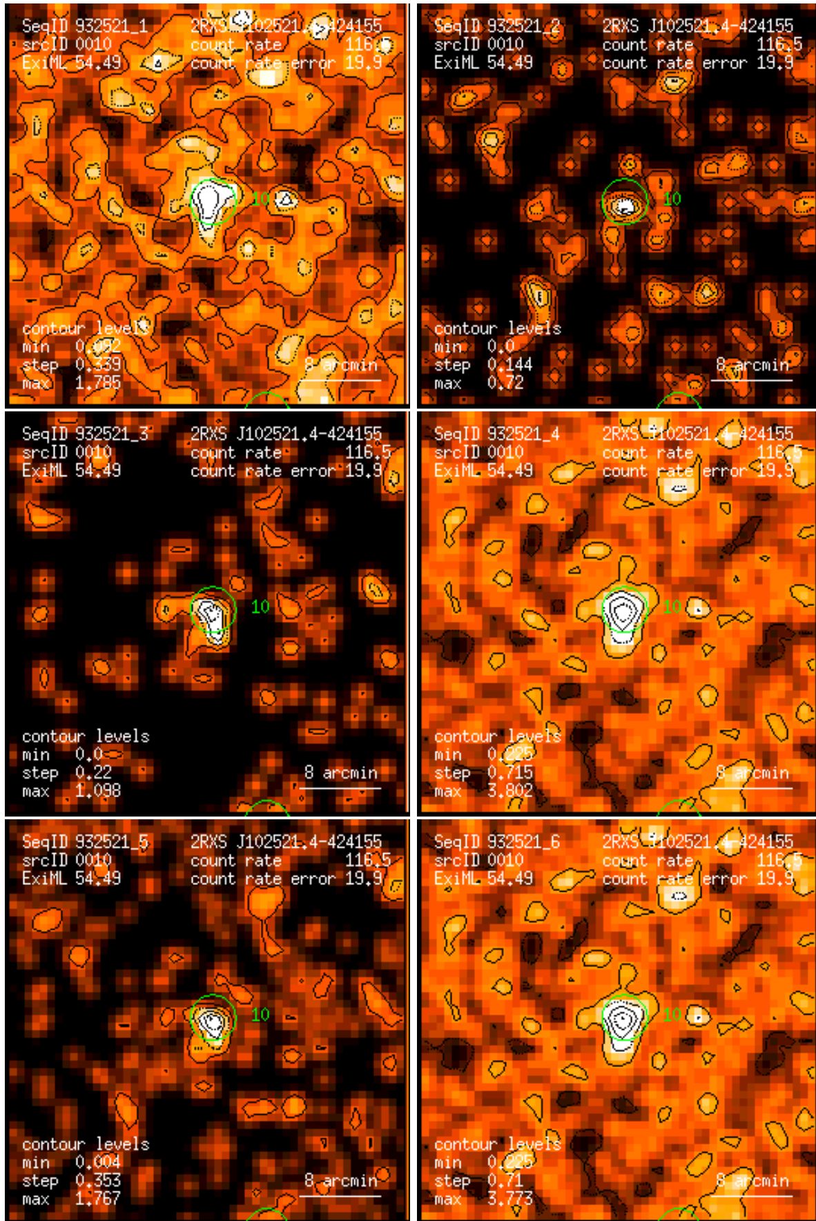
Figure 10: RASS 932521: detection 0010: band rate images, Gaussian filter: (1) PSPC channels 11 – 41, (2) 52 – 90, (3) 91 – 201, (4) 11 – 235, (5) 52 – 201, (6) 11 – 201. Broad band rates in counts/ks. Band rate contour levels in counts/ks/arcmin 2 .
