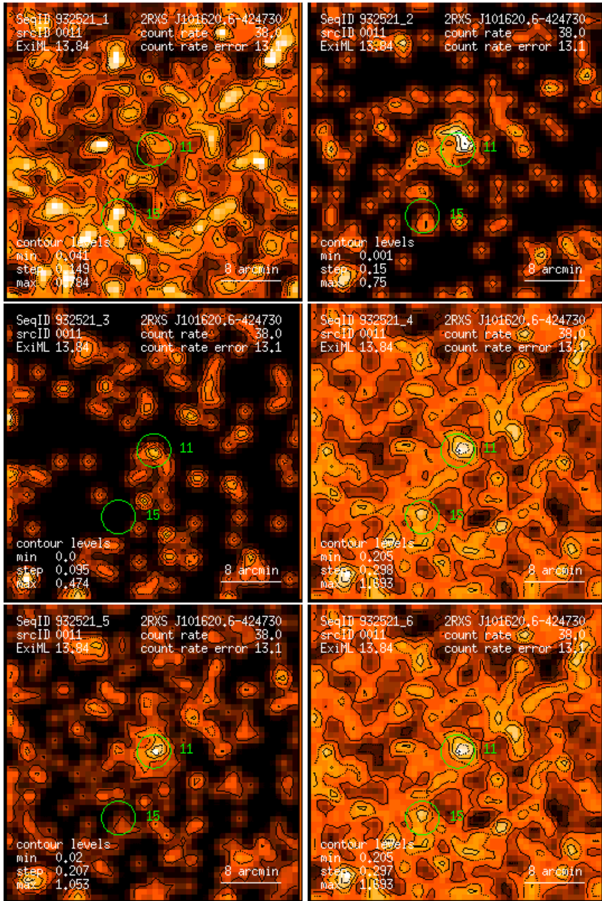
Figure 11: RASS 932521: detection 0011: band rate images, Gaussian filter: (1) PSPC channels 11 – 41, (2) 52 – 90, (3) 91 – 201, (4) 11 – 235, (5) 52 – 201, (6) 11 – 201. Broad band rates in counts/ks. Band rate contour levels in counts/ks/arcmin 2 .
