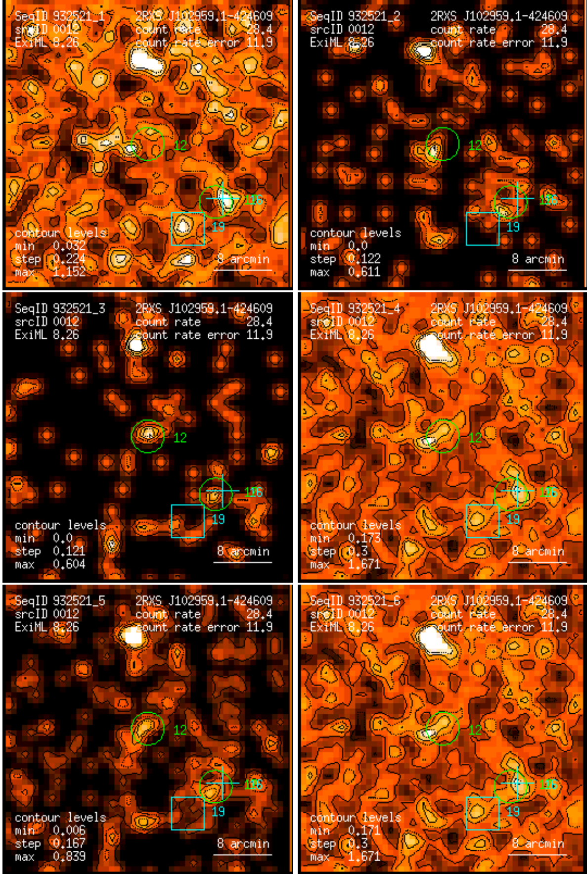
Figure 12: RASS 932521: detection 0012: band rate images, Gaussian filter: (1) PSPC channels 11 – 41, (2) 52 – 90, (3) 91 – 201, (4) 11 – 235, (5) 52 – 201, (6) 11 – 201. Broad band rates in counts/ks. Band rate contour levels in counts/ks/arcmin 2 .
