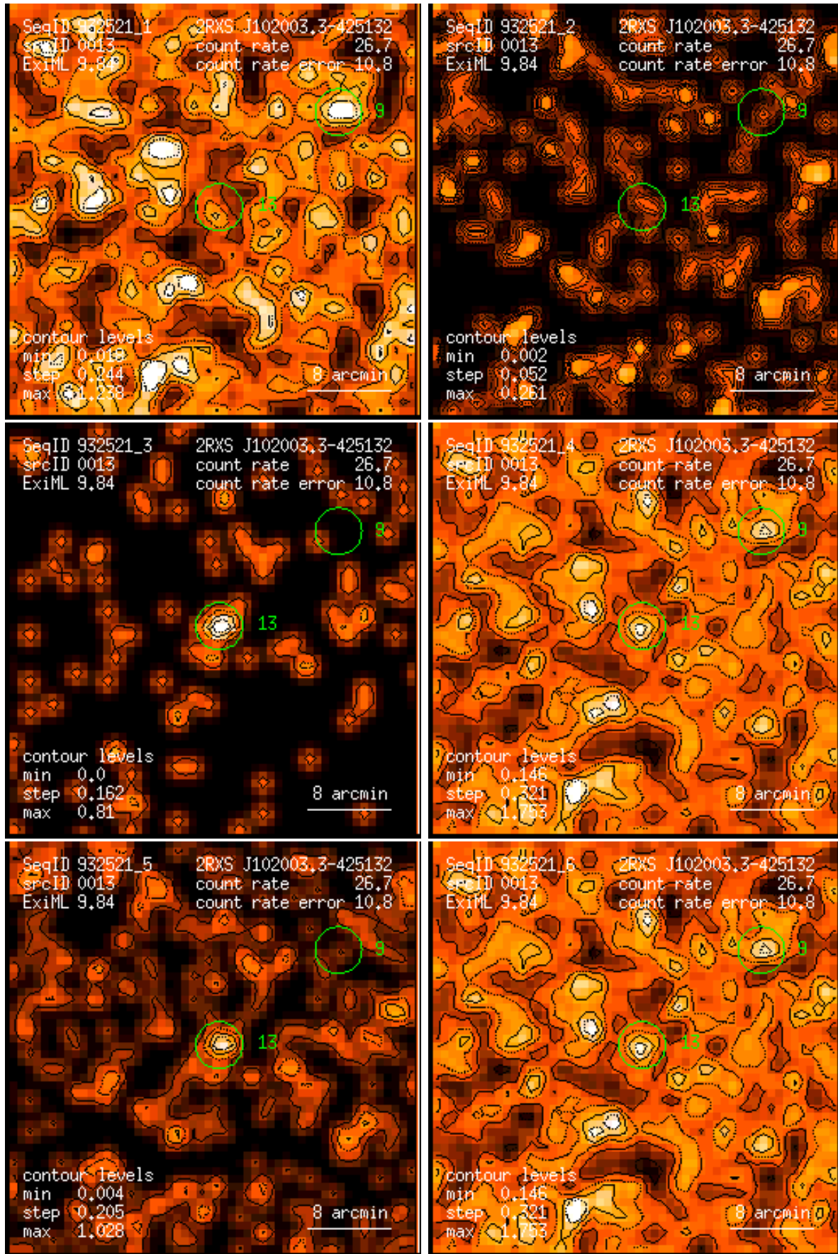
Figure 13: RASS 932521: detection 0013: band rate images, Gaussian filter: (1) PSPC channels 11 – 41, (2) 52 – 90, (3) 91 – 201, (4) 11 – 235, (5) 52 – 201, (6) 11 – 201. Broad band rates in counts/ks. Band rate contour levels in counts/ks/arcmin 2 .
