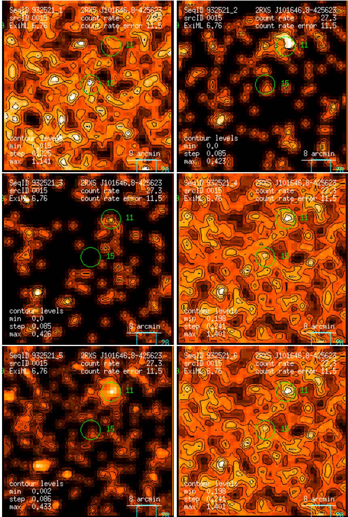
Figure 15: RASS 932521: detection 0015: band rate images, Gaussian filter: (1) PSPC channels 11 – 41, (2) 52 – 90, (3) 91 – 201, (4) 11 – 235, (5) 52 – 201, (6) 11 – 201. Broad band rates in counts/ks. Band rate contour levels in counts/ks/arcmin 2 .
