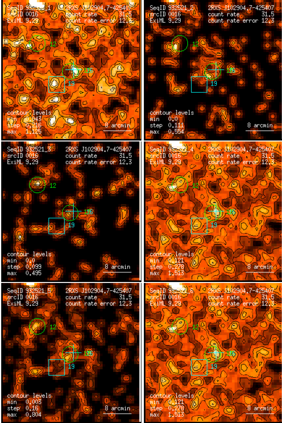
Figure 16: RASS 932521: detection 0016: band rate images, Gaussian filter: (1) PSPC channels 11 – 41, (2) 52 – 90, (3) 91 – 201, (4) 11 – 235, (5) 52 – 201, (6) 11 – 201. Broad band rates in counts/ks. Band rate contour levels in counts/ks/arcmin 2 .
