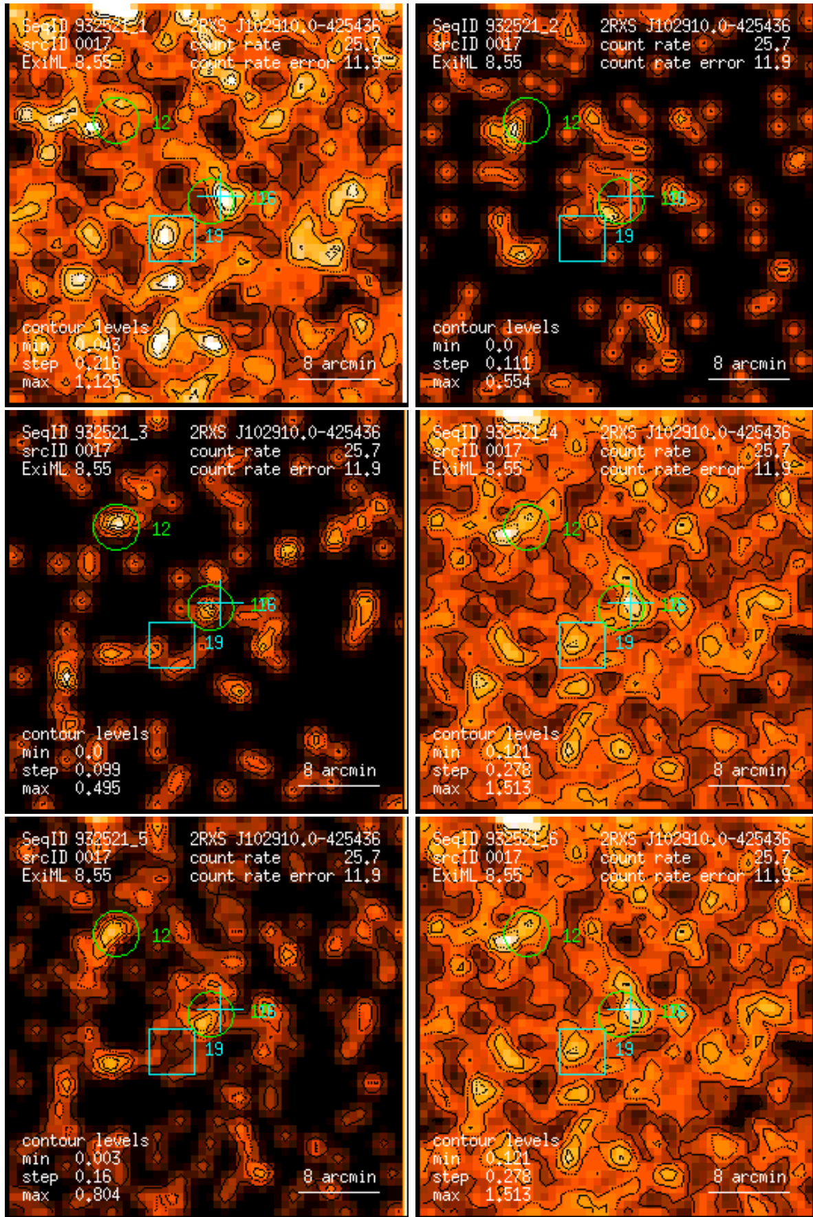
Figure 17: RASS 932521: detection 0017: band rate images, Gaussian filter: (1) PSPC channels 11 – 41, (2) 52 – 90, (3) 91 – 201, (4) 11 – 235, (5) 52 – 201, (6) 11 – 201. Broad band rates in counts/ks. Band rate contour levels in counts/ks/arcmin 2 .
