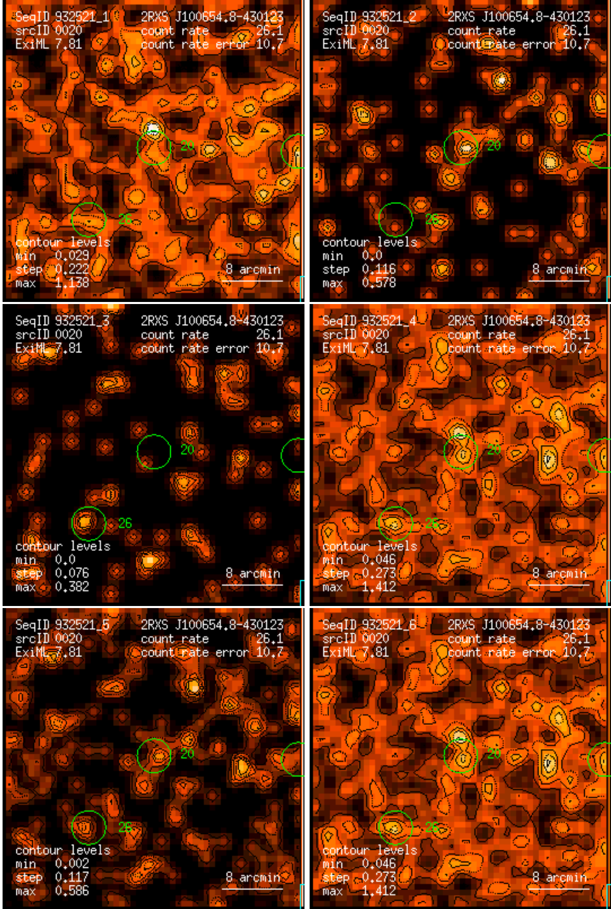
Figure 20: RASS 932521: detection 0020: band rate images, Gaussian filter: (1) PSPC channels 11 – 41, (2) 52 – 90, (3) 91 – 201, (4) 11 – 235, (5) 52 – 201, (6) 11 – 201. Broad band rates in counts/ks. Band rate contour levels in counts/ks/arcmin 2 .
