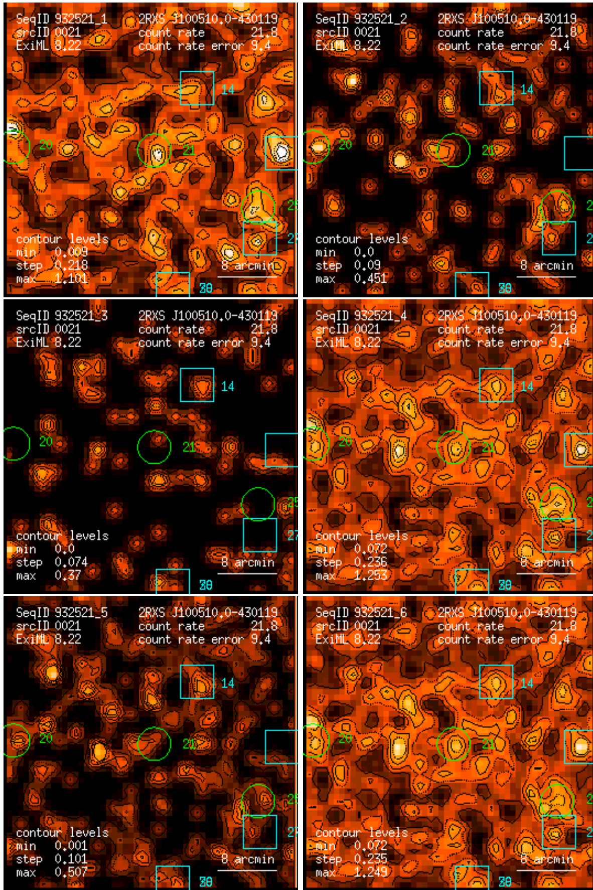
Figure 21: RASS 932521: detection 0021: band rate images, Gaussian filter: (1) PSPC channels 11 – 41, (2) 52 – 90, (3) 91 – 201, (4) 11 – 235, (5) 52 – 201, (6) 11 – 201. Broad band rates in counts/ks. Band rate contour levels in counts/ks/arcmin 2 .
