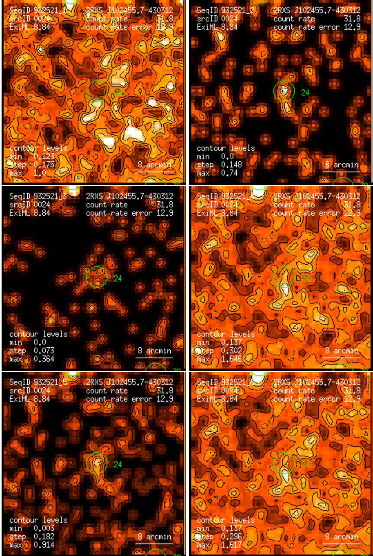
Figure 24: RASS 932521: detection 0024: band rate images, Gaussian filter: (1) PSPC channels 11 – 41, (2) 52 – 90, (3) 91 – 201, (4) 11 – 235, (5) 52 – 201, (6) 11 – 201. Broad band rates in counts/ks. Band rate contour levels in counts/ks/arcmin 2 .
