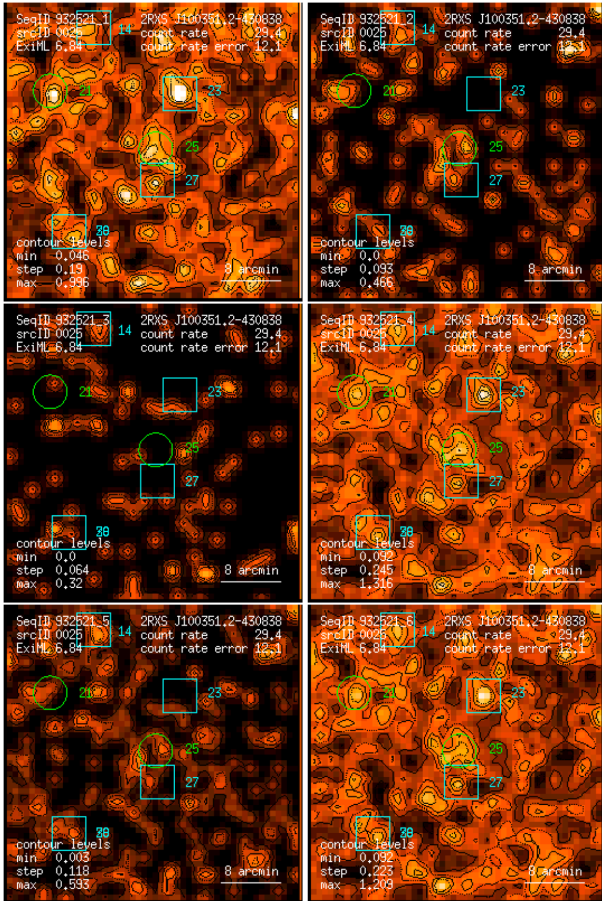
Figure 25: RASS 932521: detection 0025: band rate images, Gaussian filter: (1) PSPC channels 11 – 41, (2) 52 – 90, (3) 91 – 201, (4) 11 – 235, (5) 52 – 201, (6) 11 – 201. Broad band rates in counts/ks. Band rate contour levels in counts/ks/arcmin 2 .
