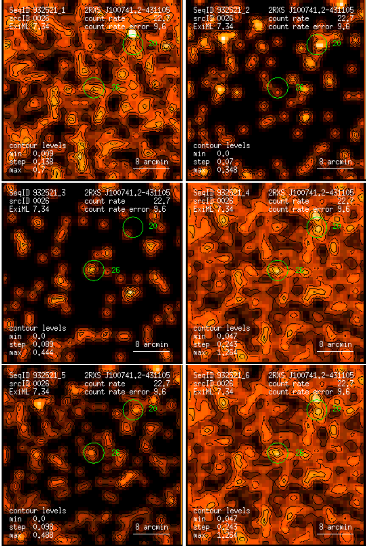
Figure 26: RASS 932521: detection 0026: band rate images, Gaussian filter: (1) PSPC channels 11 – 41, (2) 52 – 90, (3) 91 – 201, (4) 11 – 235, (5) 52 – 201, (6) 11 – 201. Broad band rates in counts/ks. Band rate contour levels in counts/ks/arcmin 2 .
