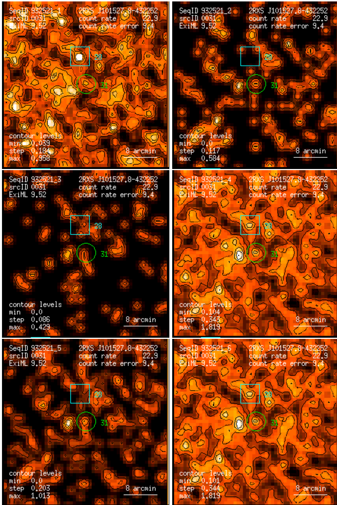
Figure 31: RASS 932521: detection 0031: band rate images, Gaussian filter: (1) PSPP channels 11 – 41, (2) 52 – 90, (3) 91 – 201, (4) 11 – 235, (5) 52 – 201, (6) 11 – 201. Broad band rates in counts/ks. Band rate contour levels in counts/ks/arcmin 2 .
