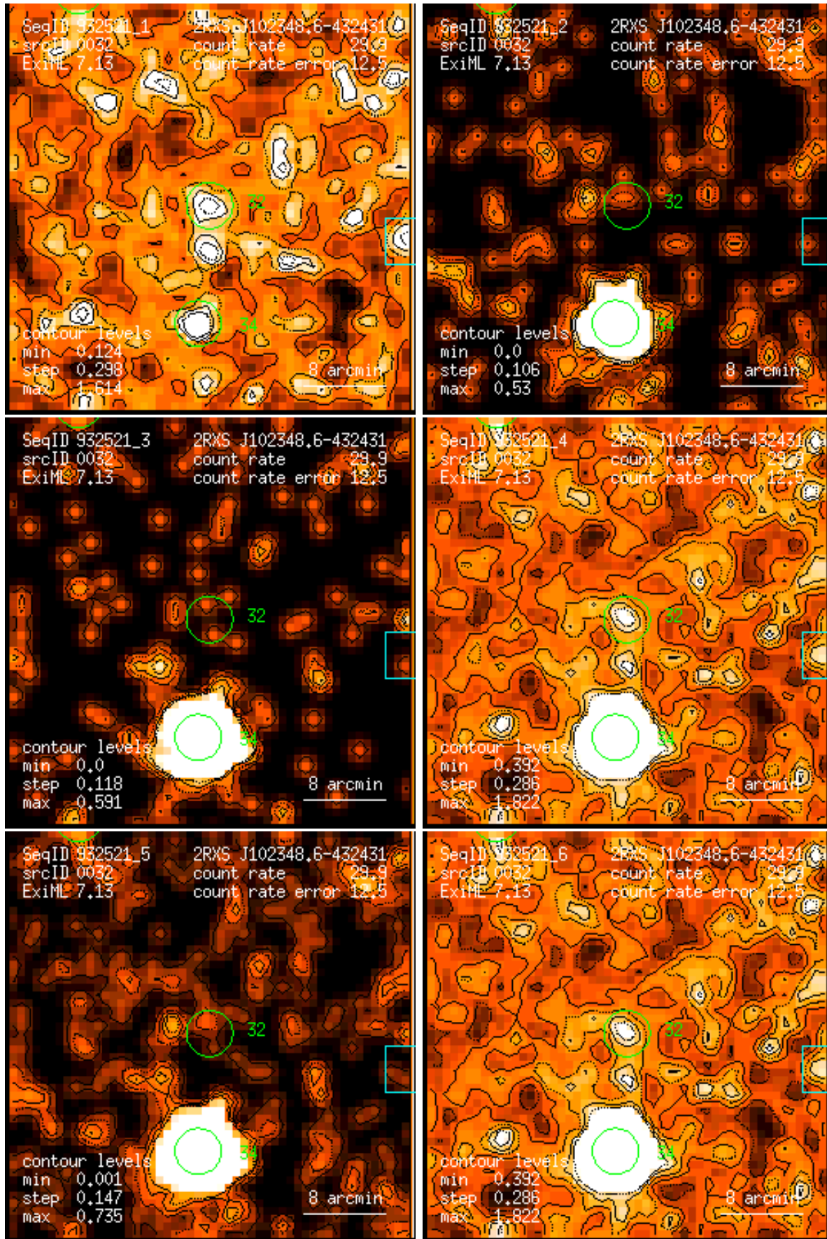
Figure 32: RASS 932521: detection 0032: band rate images, Gaussian filter: (1) PSPC channels 11 – 41, (2) 52 – 90, (3) 91 – 201, (4) 11 – 235, (5) 52 – 201, (6) 11 – 201. Broad band rates in counts/ks. Band rate contour levels in counts/ks/arcmin 2 .
