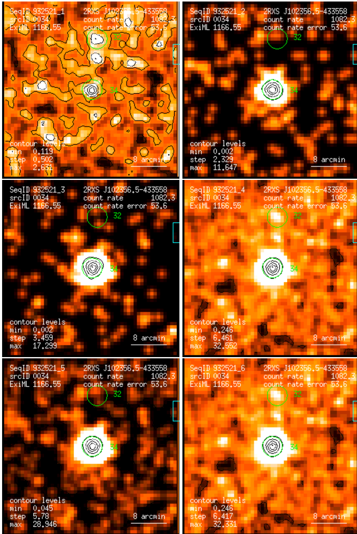
Figure 34: RASS 932521: detection 0034: band rate images, Gaussian filter: (1) PSPC channels 11 – 41, (2) 52 – 90, (3) 91 – 201, (4) 11 – 235, (5) 52 – 201, (6) 11 – 201. Broad band rates in counts/ks. Band rate contour levels in counts/ks/arcmin 2 .
