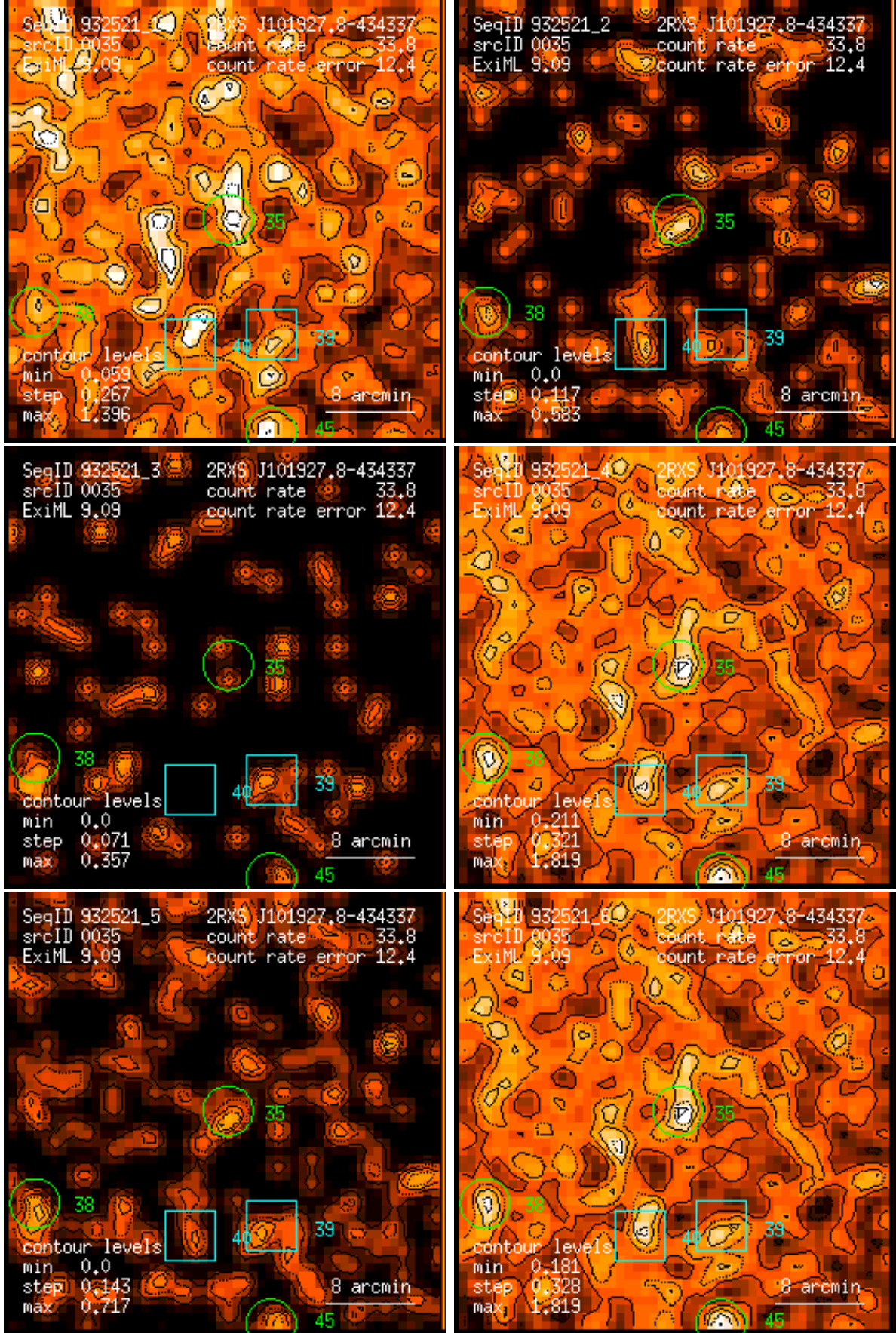
Figure 35: RASS 932521: detection 0035: band rate images, Gaussian filter: (1) PSPC channels 11 – 41, (2) 52 – 90, (3) 91 – 201, (4) 11 – 235, (5) 52 – 201, (6) 11 – 201. Broad band rates in counts/ks. Band rate contour levels in counts/ks/arcmin 2 .
