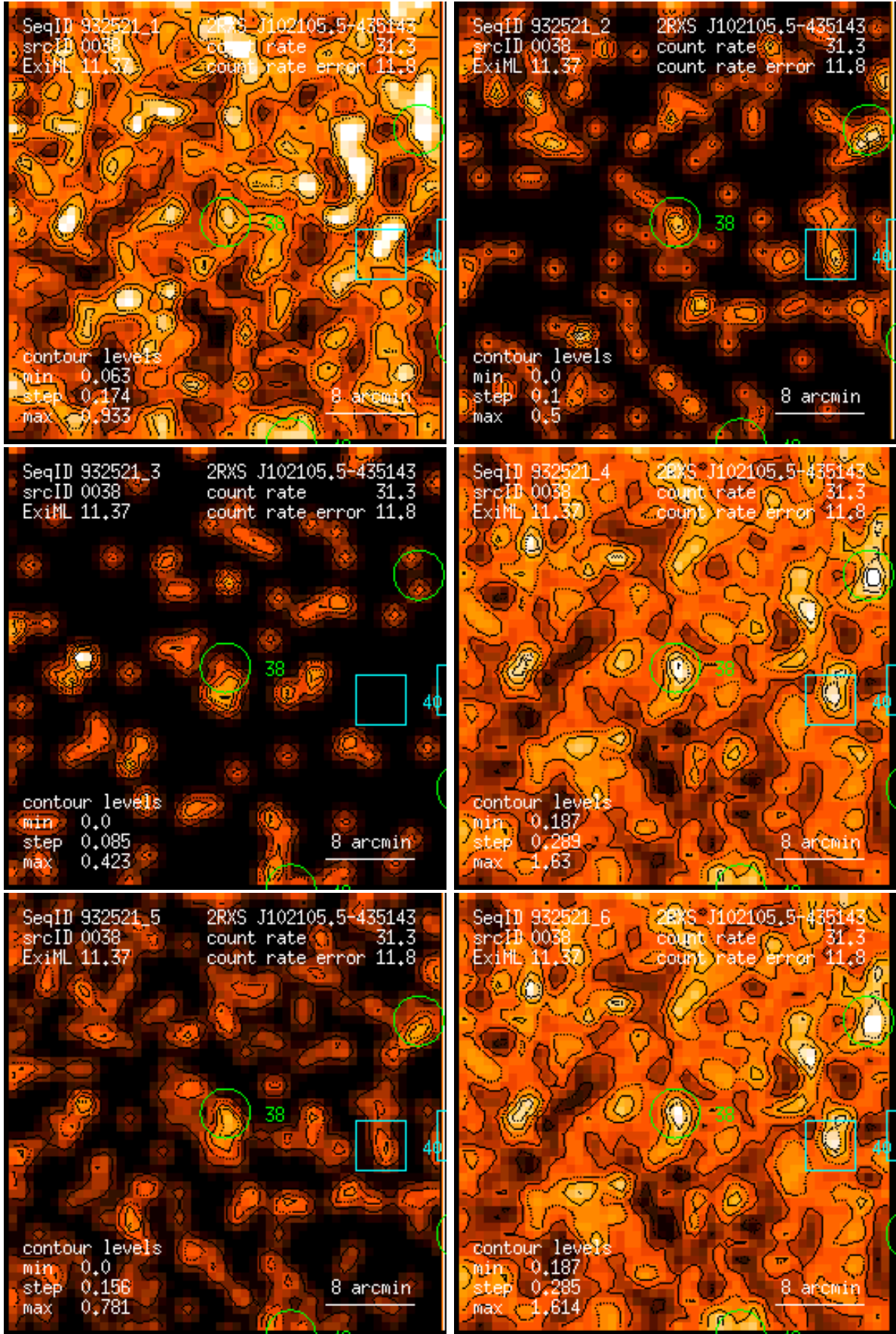
Figure 38: RASS 932521: detection 0038: band rate images, Gaussian filter: (1) PSPC channels 11 – 41, (2) 52 – 90, (3) 91 – 201, (4) 11 – 235, (5) 52 – 201, (6) 11 – 201. Broad band rates in counts/ks. Band rate contour levels in counts/ks/arcmin 2 .
