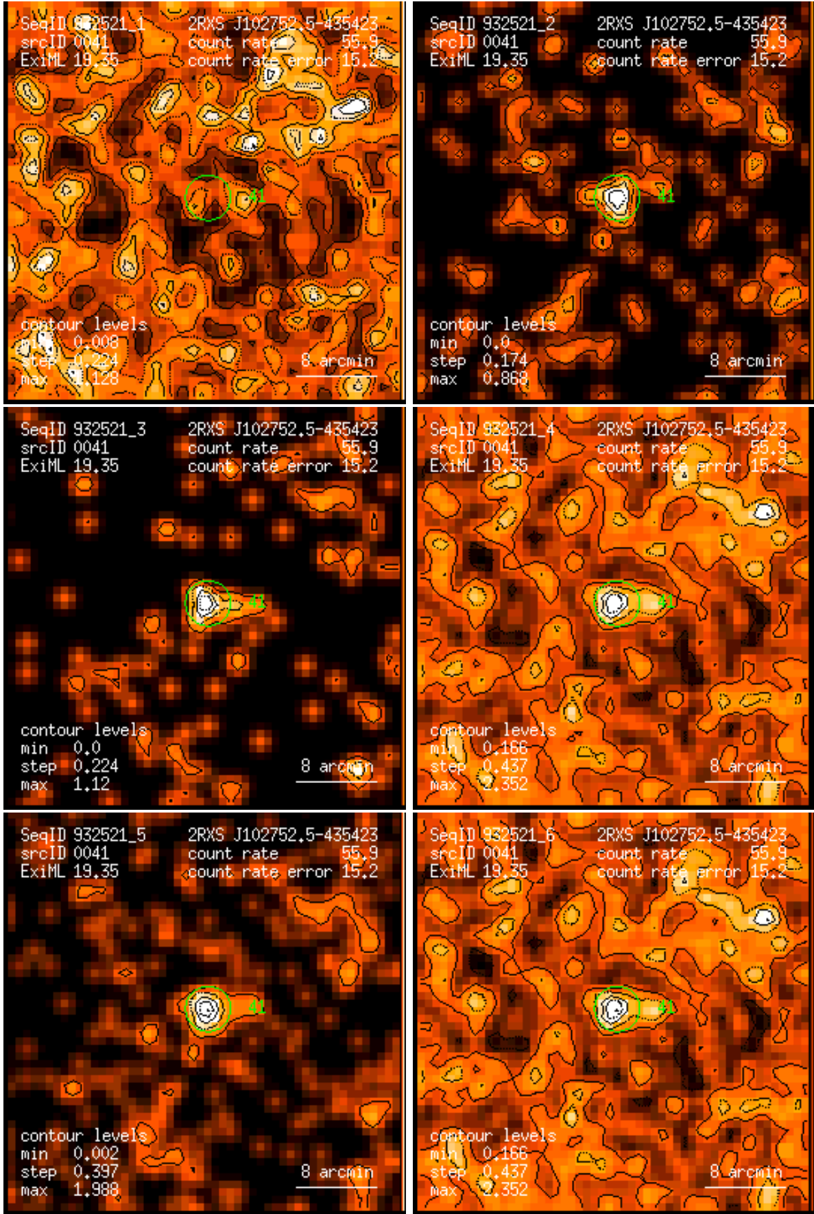
Figure 41: RASS 932521: detection 0041: band rate images, Gaussian filter: (1) PSPC channels 11 – 41, (2) 52 – 90, (3) 91 – 201, (4) 11 – 235, (5) 52 – 201, (6) 11 – 201. Broad band rates in counts/ks. Band rate contour levels in counts/ks/arcmin 2 .
